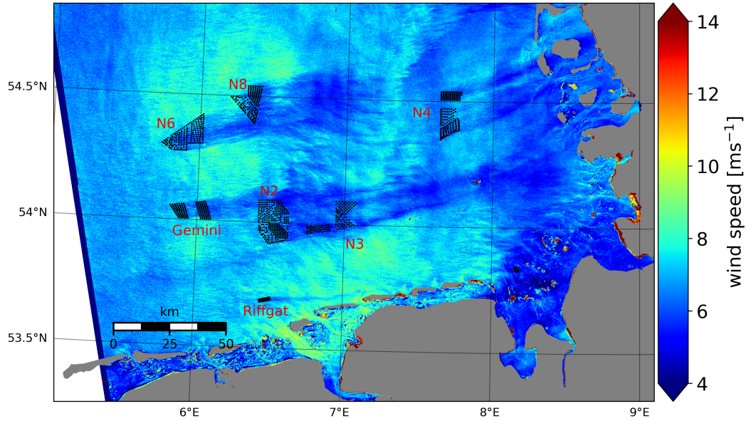
Figure 1. 10-m wind speed derived from Sentinel-1A SAR (Contains modified Copernicus Sentinel data [2021]) data acquired on 11 September 2021 at 17:17 UTC. Black dots represent wind turbines; names of wind farms and clusters are labelled in red. The wind direction is from West. Powered by Esri.
