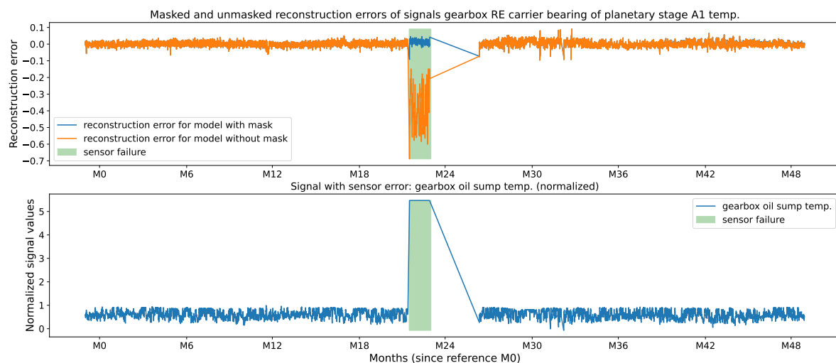
Figure 6. Sensor-Gearbox oil sump temperature (bottom plot) sensor failure (bottom plot, green box) and its impact (top plot) on the reconstruction error of a different signal-gearbox RE carrier bearing of planetary stage A1 temperature (top plot) without (top plot, orange curve) and with (top plot, blue curve) masking for of the sensor error. The data originates from turbine 1 of WF1.
