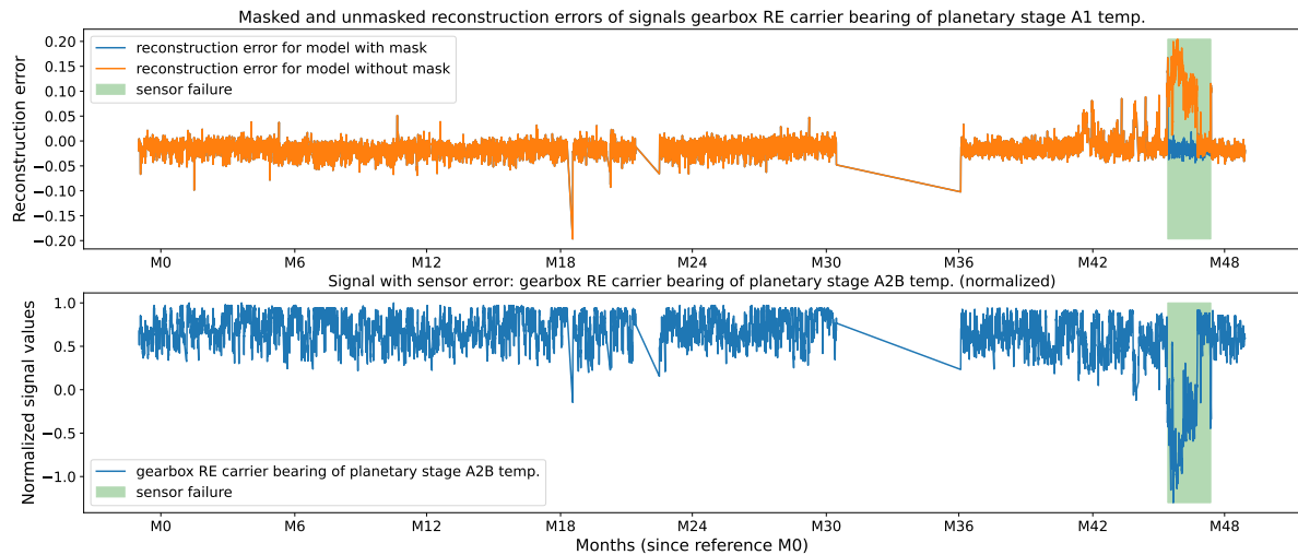
Figure 7. Sensor-Gearbox RE carrier bearing of planetary stage A2B temperature (bottom plot) sensor failure (bottom plot, green box) and its impact (top plot) on the reconstruction error of a different signal-gearbox RE carrier bearing of planetary stage A1 temperature (top plot) without (top plot, orange curve) and with (top plot, blue curve) masking for of the sensor error. The data originates from turbine 21 of WF1.
