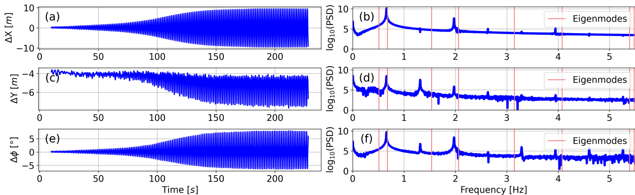
Figure 7. Edgewise-vibration-Vibration ramp up of the FLEX37 setup in the edge-wise (a)time-, flapwise (c) and torsional component (e). Frequency contributions of the respective components are shown in (b)frequency-domain, (d) and (f). The vertical lines indicate the blade's eigenmodes. From low to high, the first, third and fifth frequencies correspond to the first three flapwise eigenfrequencies and the second, fourth and sixth correspond to the first three edgewise eigenfrequencies. The seventh frequency represents the first torsional natural frequency.
