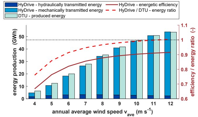
Figure 15. Comparison of AEP estimation between standard DTU 10MW turbine and HyDrive drivetrain. Energetic efficiency of HyDrive drivetrain (red) and relative energy ratio (red-dashed) between HyDrive and DTU turbine. Direct transmission at rated wind speed and rotor-side power-split.
