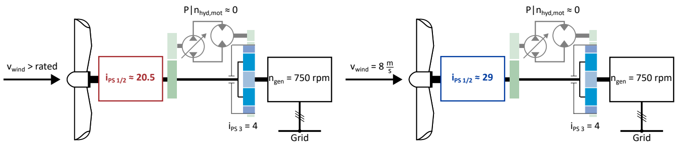
a) Direct transmission at 11.4 \frac{m}{s} (rated wind speed).
