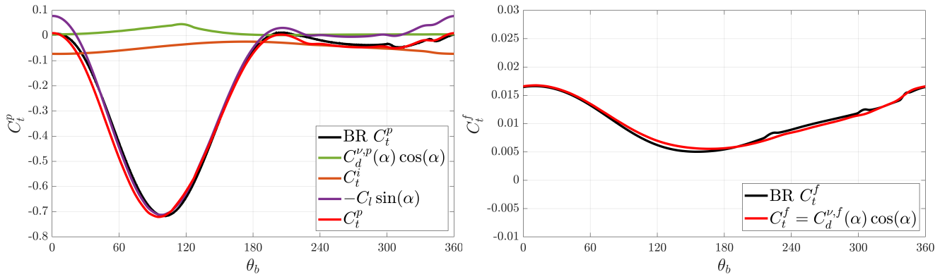
Figure 12. VAT with NACA0015 airfoil attached at x_p = c/4 and operating at TSR = 3.25 : comparison between the ALM with m_{c/4} and f_t^i explicitly enforced (red) and the reference wall-resolved simulation (black) of the pressure contribution C_t^p (with its components) and of the friction contribution C_t^f to the tangential force coefficient.
