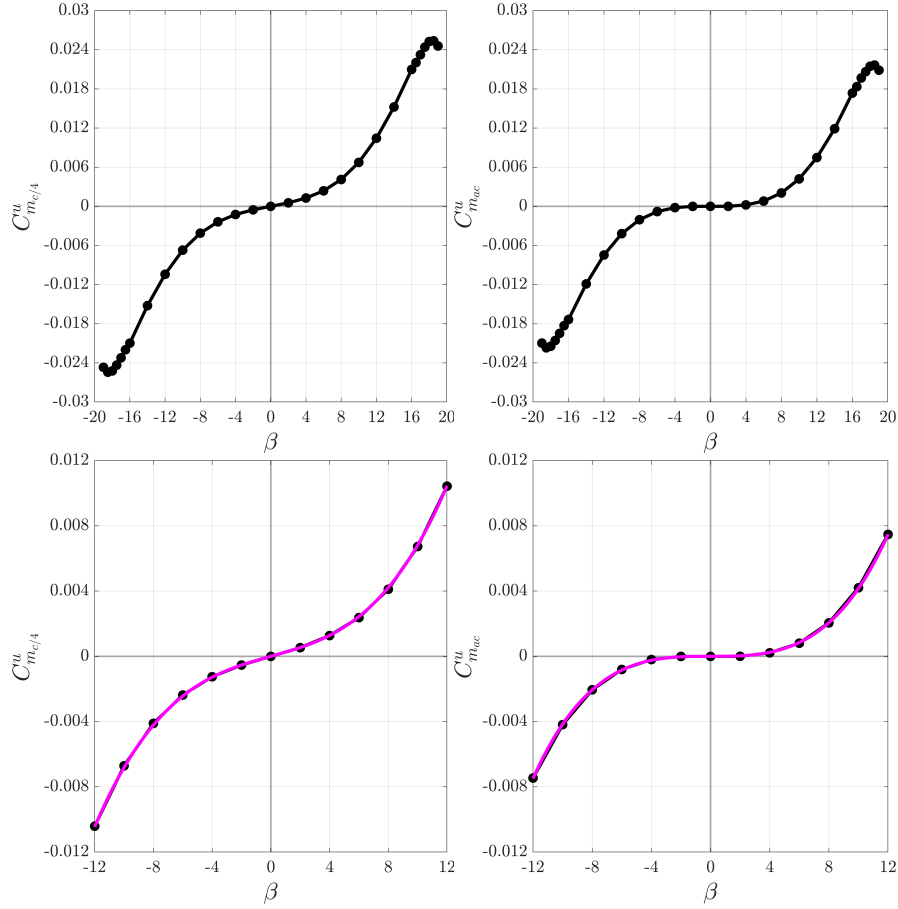
Figure A2. Coefficients C_{m_{nac}}^u and C_{m_{c/4}}^u as a function of the angle of attack \beta : data for the complete range (top); data for the range |\beta| \leq 12 deg (bottom) and with the mathematical fit (magenta).
