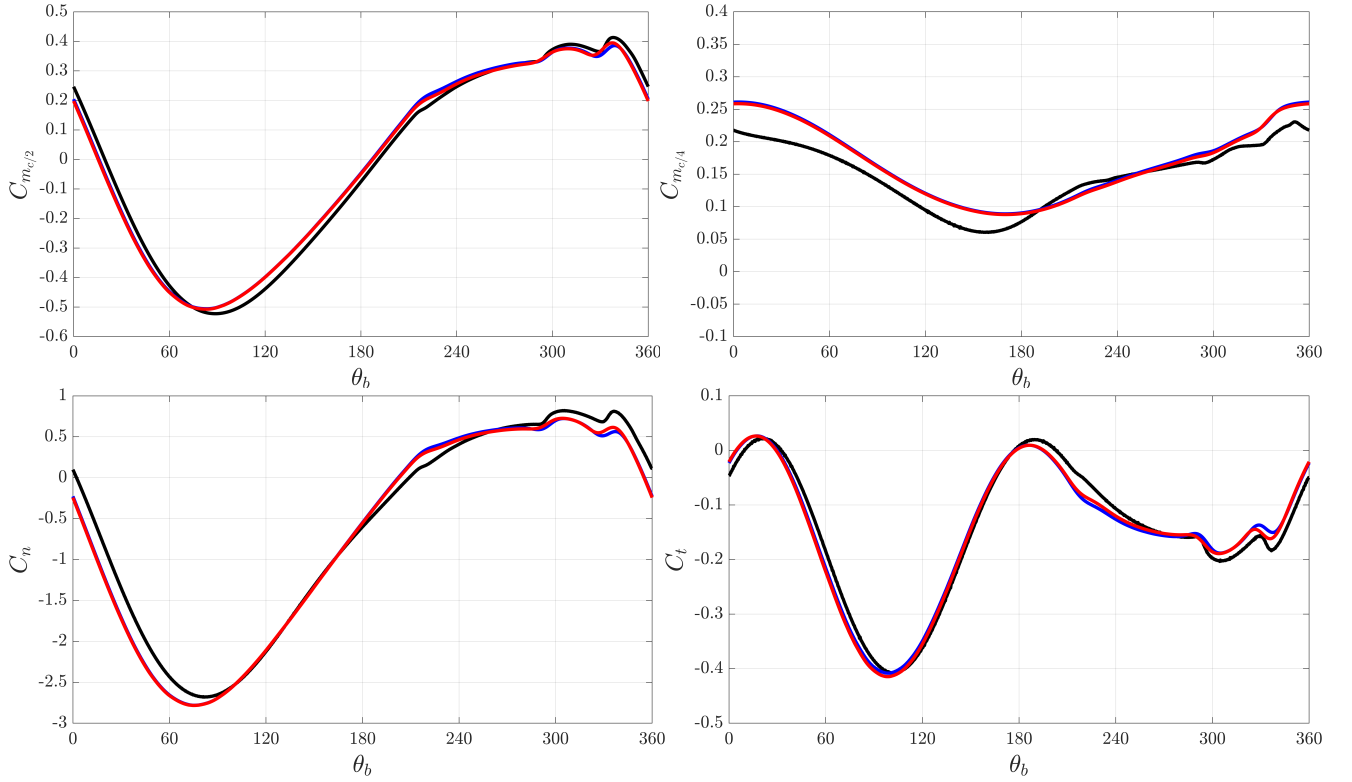
Figure 14. VAT with NACA0015 airfoil attached at x_p = c/2 and operating at TSR = 3.25 : comparison between the ALM with m_{c/4} , f_t^i and f_n^i explicitly enforced (red), the ALM without m_{c/4} , f_t^i and f_n^i explicitly enforced (blue) and the reference wall-resolved simulation (black) of C_{m_{c/2}} , C_{m_{c/4}} , C_n and C_t . Both ALM cases are centered at c/4 .
