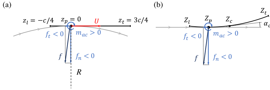
Figure 5. (a): Schematic of a flat plate attached at x_p = c/4 and without pitch angle in the z -plane (solid black) and a background flow with curved streamlines (light grey). (b): transformed tilted cambered plate in the Z -plane in a uniform background flow. Note: the flow curvature was here exaggerated for clarity, using a too large value of c/R = 1/2 .
