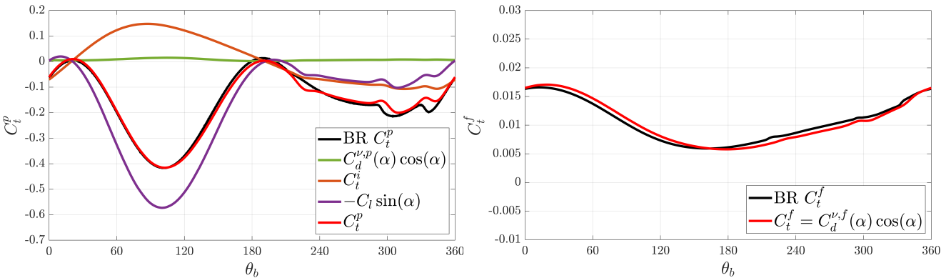
Figure 19. VAT with NACA0015 airfoil attached at x_p = c/2 and operating at TSR = 3.25 : comparison between the ALM with m_{c/2} and f_t^i explicitly enforced (red) and the reference wall-resolved simulation (black) of the pressure contribution C_t^p (with its components) and of the friction contribution C_t^f to the tangential force coefficient. The ALM is centered at x_p = c/2 .
