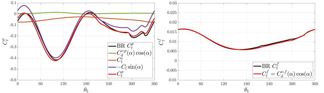
Figure 16. VAT with NACA0015 airfoil attached at x_p = c/2 and operating at TSR = 3.25 : comparison between the ALM with m_{c/4} , f_t^i and f_n^i explicitly enforced (red) and the reference wall-resolved simulation (black) of the pressure contribution C_t^p (with its components) and of the friction contribution C_t^f to the tangential force coefficient. The ALM is centered at c/4 .
