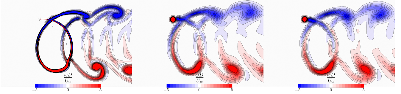
Figure 13. Vorticity field for the wall-resolved simulation (left), the ALM simulation without m_{c/4} enforced (center) and the ALM simulation with m_{c/4} enforced (right).
