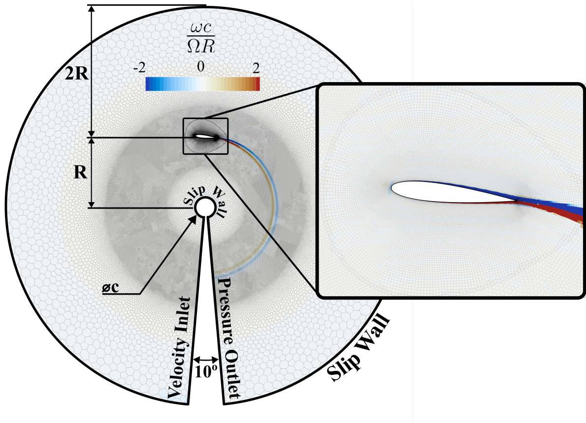
Figure B1. Simulation setup and key-hole mesh used for the simulation of the NACA0015 airfoil in rotation with c/R = 2/7 . Case with airfoil attached at mid-chord ( x_p = c/2 ) and tilting angle \alpha_p = 6 deg. A zoom on the body-fitted mesh around the airfoil is also shown.
