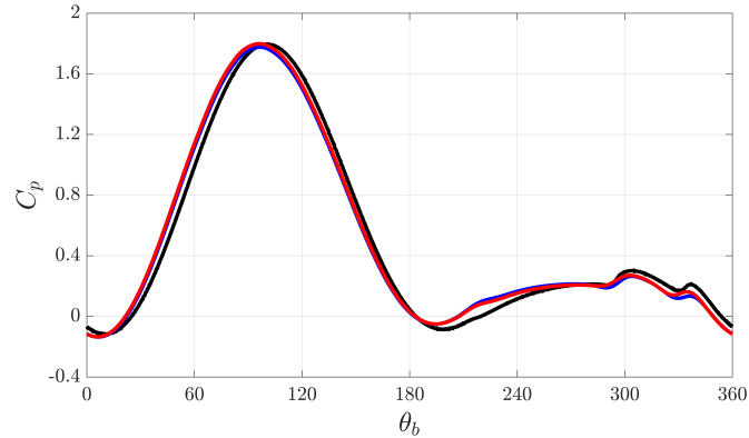
Figure 15. VAT with NACA0015 airfoil attached at x_p = c/2 and operating at TSR = 3.25 : comparison between the results of the ALM with m_{c/4} , f_t^i and f_n^i explicitly enforced (red), the ALM without m_{c/4} , f_t^i and f_n^i explicitly enforced (blue) and the reference wall-resolved simulation (black) of C_p . Both ALM cases are centered at c/4 .
