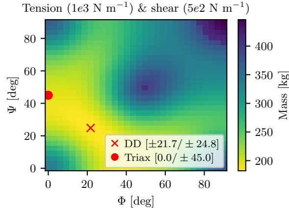
Figure 6. Optimized mass distribution for the \overline{DD} - \overline{DD} laminate under combined tension and shear loading.
