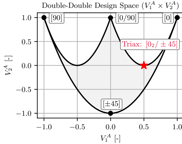
Figure 3. Design space of DD DD laminates in the V_1^A – V_2^A plane.
