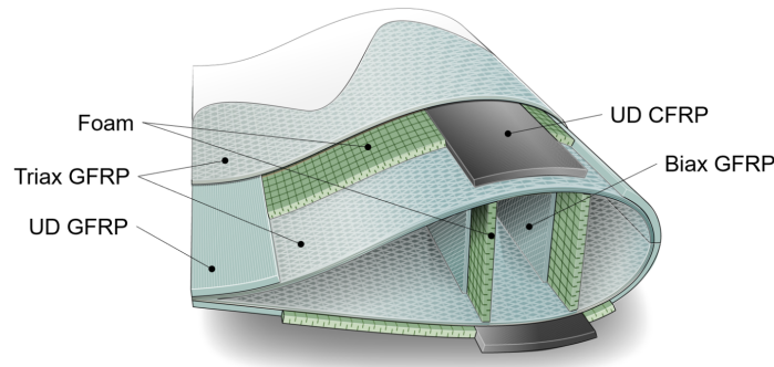
Figure 1. IEA-IEA 15 MW structural concept. Source: (Werthen et al., 2023).
