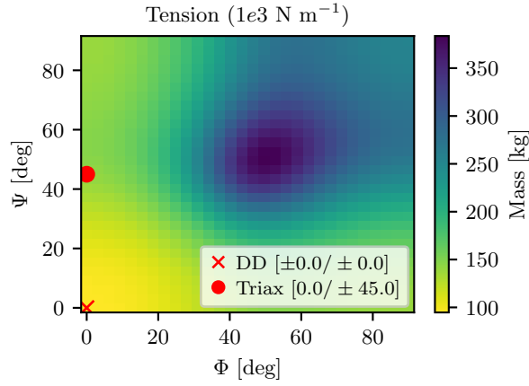
Figure 4. Optimized mass distribution for the DD laminate under axial tension.
