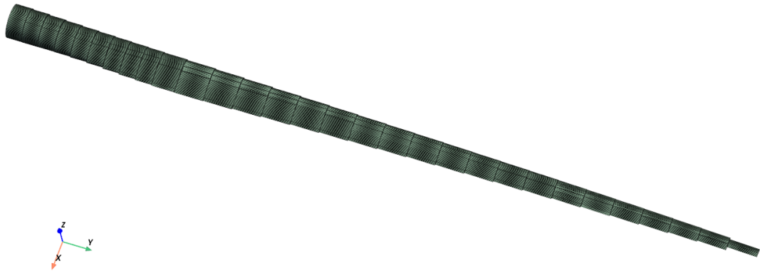
Figure 14. Structural discretization of the CRC-15-240 blade in PreDoCS .
