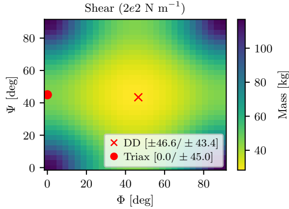
Figure 5. Optimized mass distribution for the DD -DD laminate under pure shear loading.
