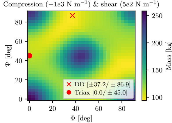
Figure 7. Optimized mass distribution for the \overline{DD} - \overline{DD} laminate under combined compression and shear loading.
