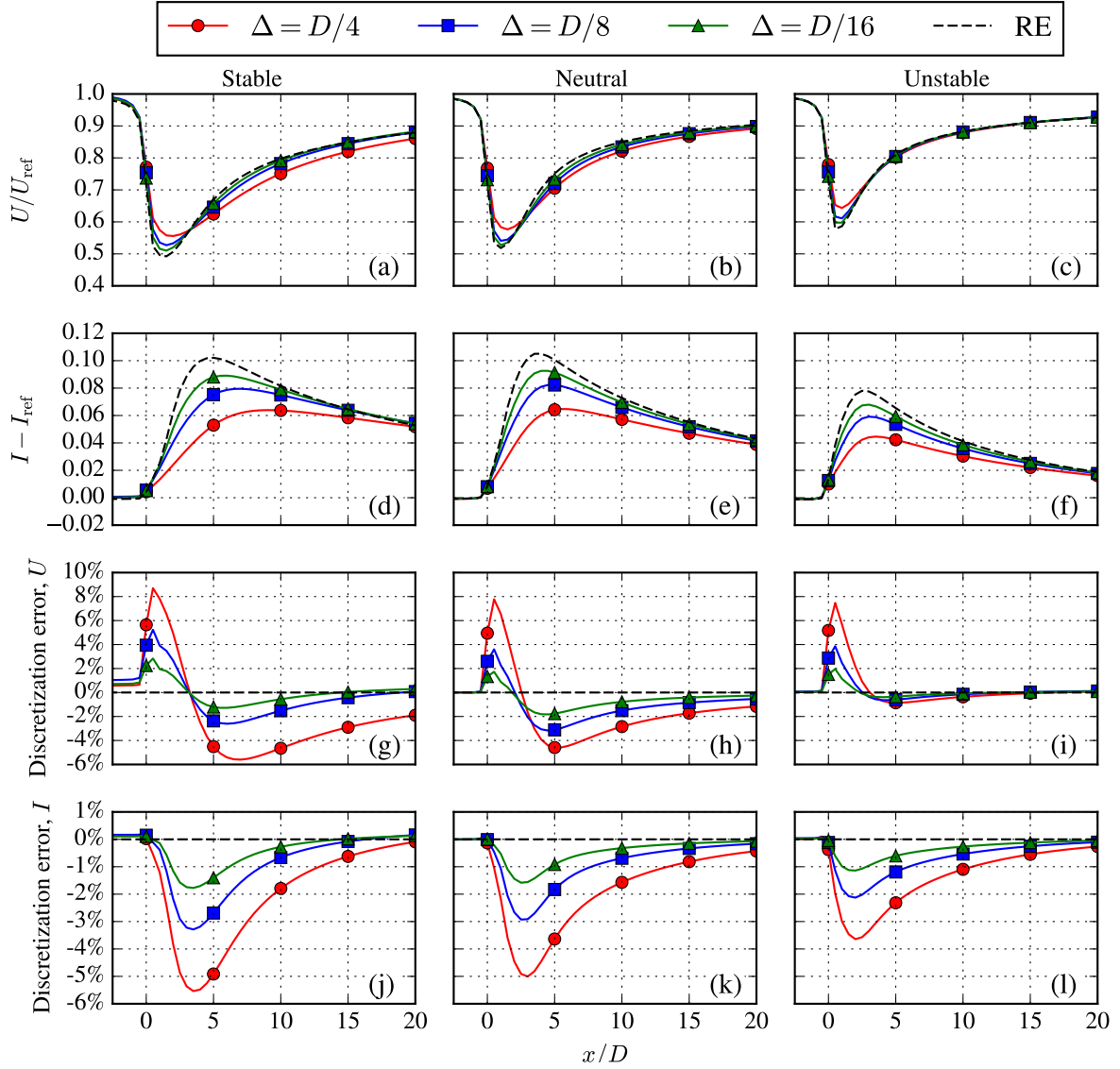
Figure C1. Influence of grid spacing on RANS-AD single wake results in terms of rotor averaged streamwise velocity (a-c) and wake-added TI (d-f), and corresponding discretization errors (g-l), for different stability cases. RE is Richardson extrapolated value.
