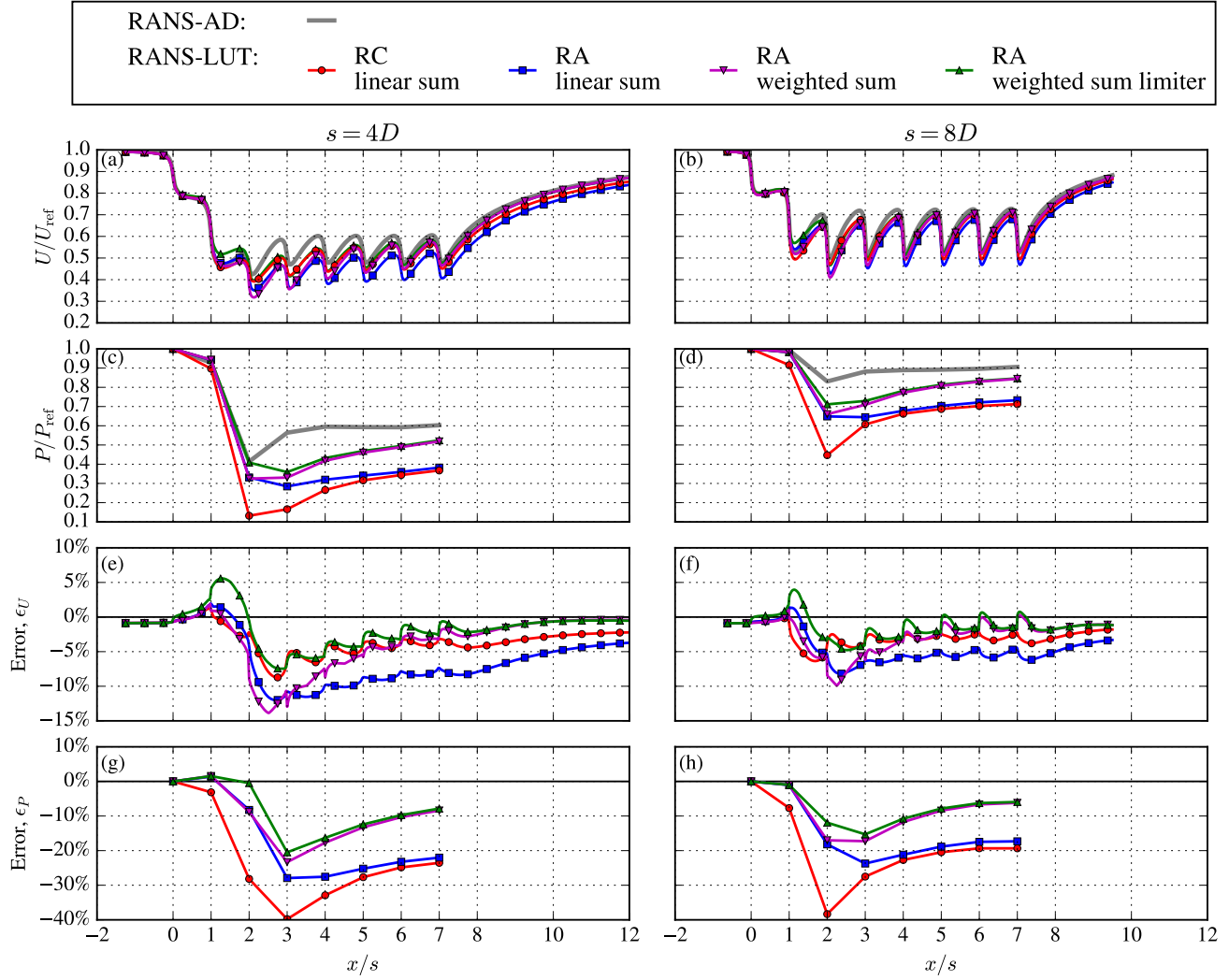
Figure B1. Rotor averaged streamwise velocity (a-b) and wind turbine power (c-d), and corresponding model errors (e-h), in a turbine row with 4D and 8D turbine spacing, U_{\text{ref}} = 14 \text{ ms}^{-1} (variable C_T ) and stable conditions. Results are shown for different rotor averaging and superposition methods.
