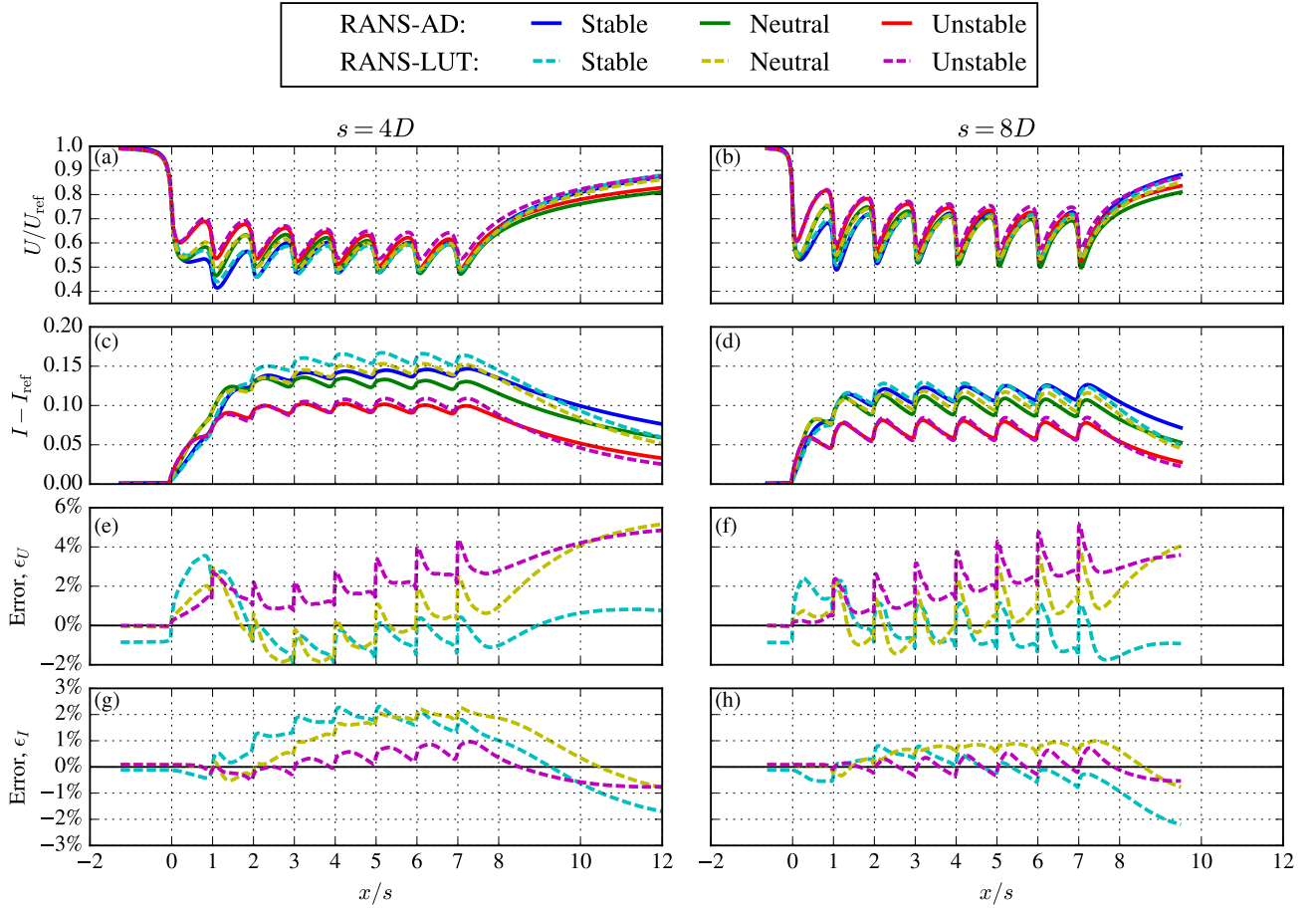
Figure 3. Rotor-averaged streamwise velocity (a-b) and wake-added TI (c-d), and corresponding model errors (e-h), in a turbine row with 4D and 8D turbine spacing, and U_{\text{ref}} = 11 \text{ ms}^{-1} (constant C_T = 0.8 ).
