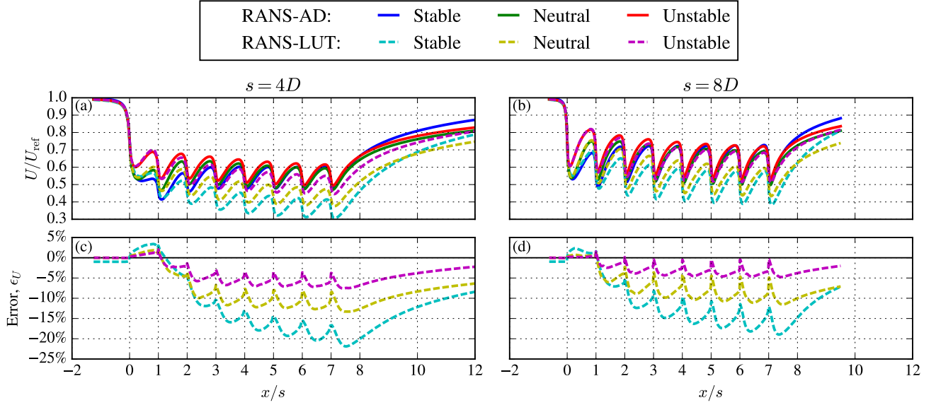
Figure 7. Rotor averaged streamwise velocity (a-b), and corresponding model errors (c-d) in a turbine row with 4D and 8D turbine spacing, and U_{\text{ref}} = 11 \text{ ms}^{-1} (constant C_T ), without wake-added TI LUTs.
