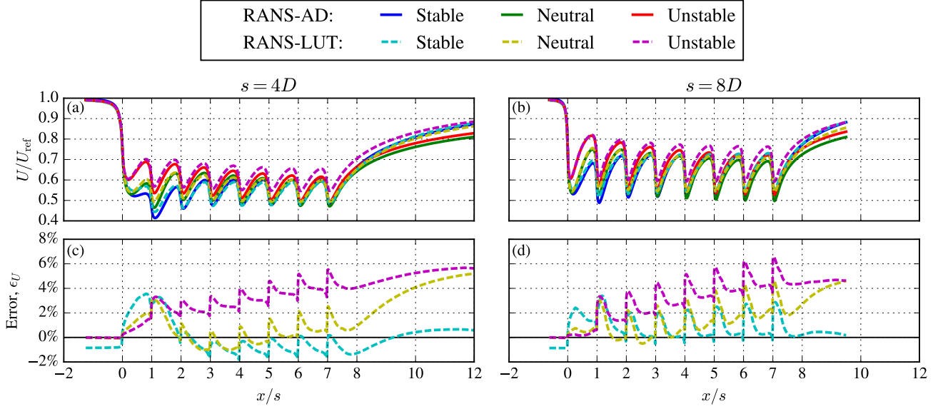
Figure 5. Rotor averaged streamwise velocity (a-b) for prescribed wake-added TI values from RANS-AD, and corresponding model errors (c-d), in a turbine row with 4D and 8D turbine spacing, and U_{\text{ref}} = 11 \text{ ms}^{-1} (constant C_T = 0.8 ).
