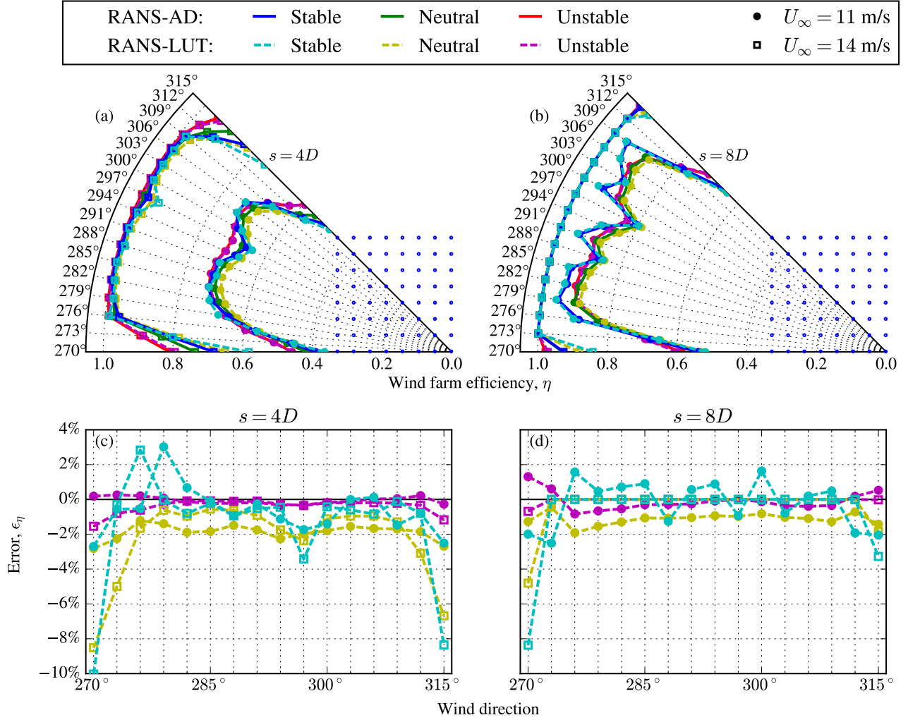
Figure 9. Wind farm efficiency (a-b) and corresponding RANS-LUT model error (c-d), for 8 \times 8 wind farm with 4D (a, c) and 8D (b, d) turbine spacing, and U_{\text{ref}} = 11 \text{ ms}^{-1} and U_{\text{ref}} = 14 \text{ ms}^{-1} .
