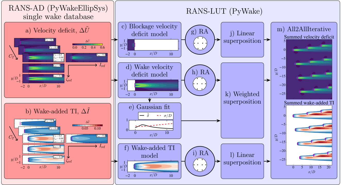
Figure 2. Overview of RANS-AD single wake database (a-b) and workflow of the proposed RANS-LUT surrogate model (c-m). Contour plots depict the flow at hub height and magenta rectangle illustrates the location of the AD model. (g-i) are rotor-averaging (RA) operators. An example of a final result of the iterative method All2AllIterative is shown in (m).
