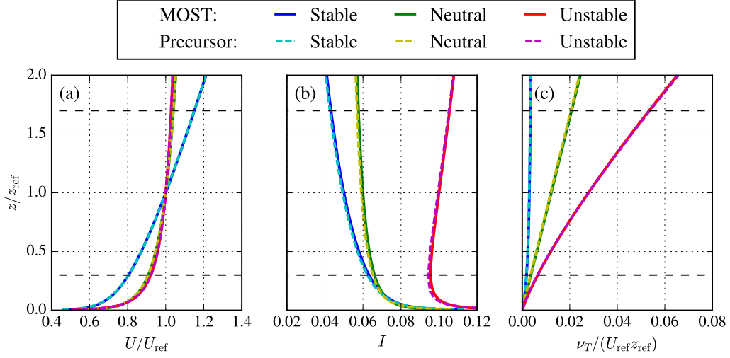
Figure 1. Normalized inflow profiles of wind speed (a), turbulence intensity (b) and eddy viscosity (c) as computed by the 1D precursor and compared with MOST. Rotor area of the NREL-5MW reference turbine is depicted with horizontal dashed lines.
