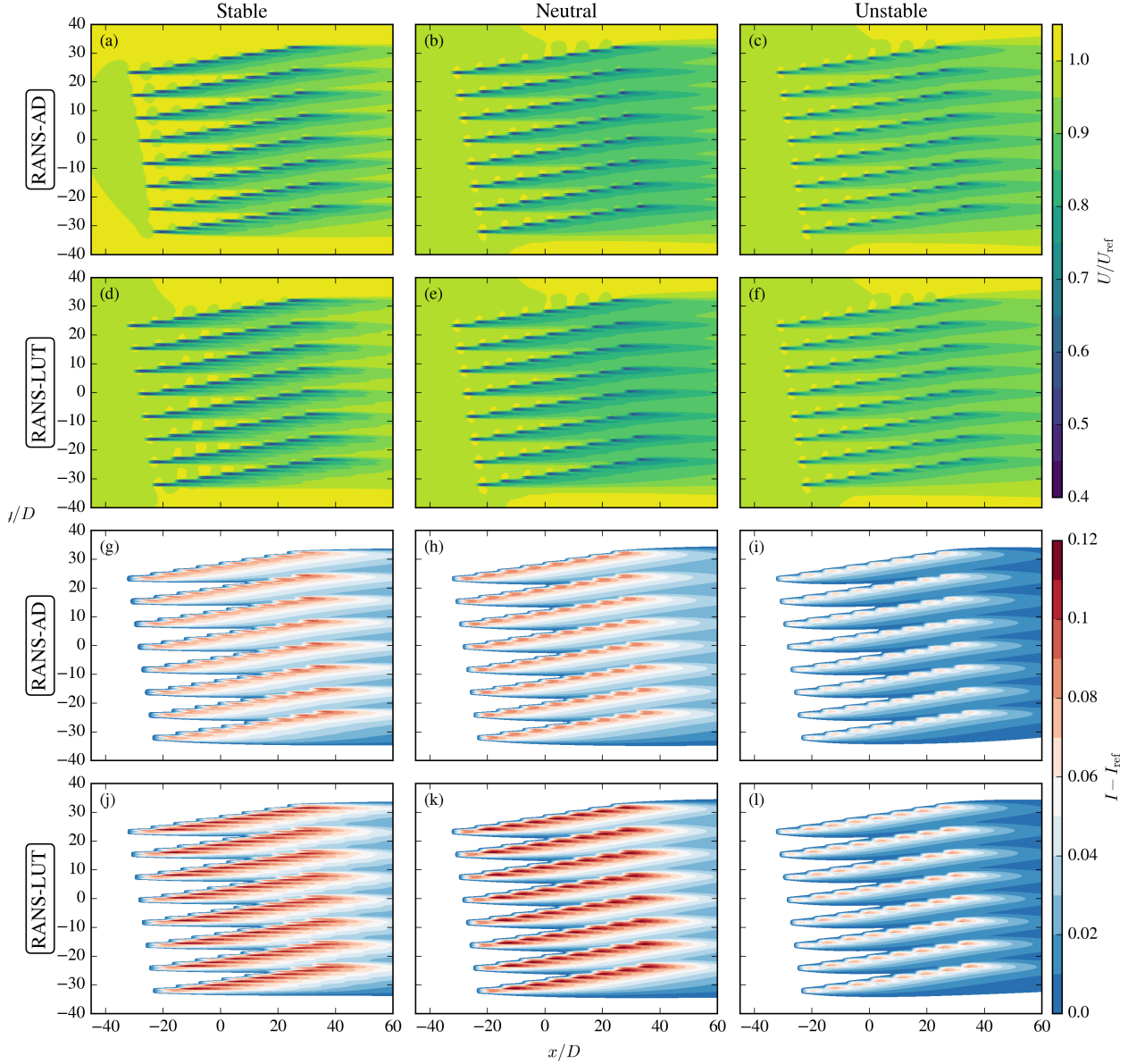
Figure 6. Flow at hub height in terms of streamwise velocity (a-f) and wake-added TI (g-l), for RANS-AD and RANS-LUT models, a wind farm with 8D turbine spacing, and U_{\text{ref}} = 11 \text{ ms}^{-1} (constant C_T = 0.8 ).
