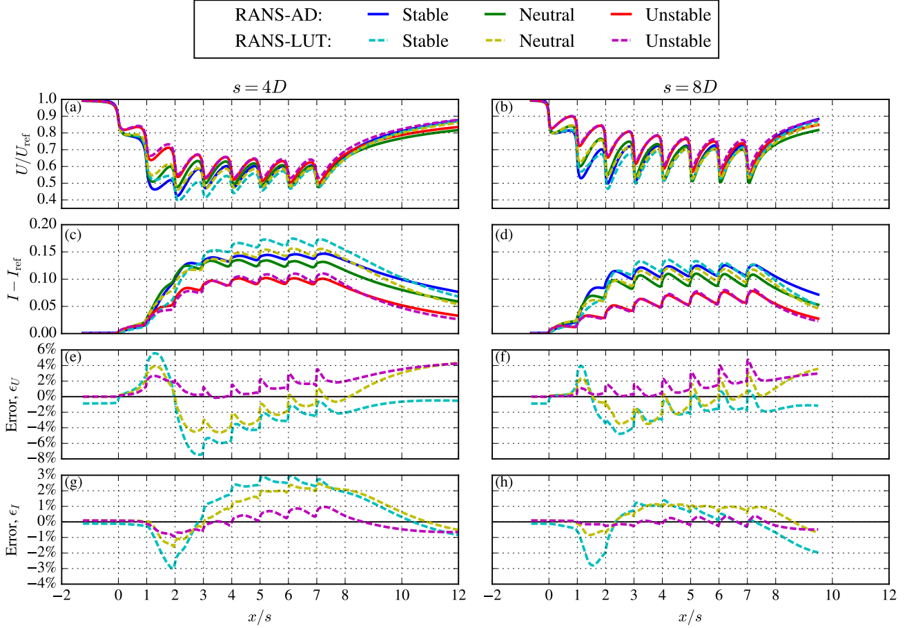
Figure 4. Same as Fig. 3 for U_{\text{ref}} = 14 \text{ ms}^{-1} (variable C_T ).
