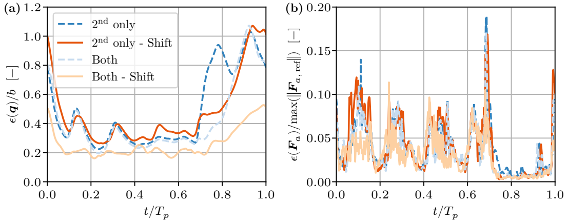
Figure 20. Six-cycle averaged error in position \epsilon(\mathbf{q}) = RMS(\|\mathbf{q} - \mathbf{q}_{ref}\|) (a) and forces \epsilon(\mathbf{F}_a) = RMS(\|\mathbf{F}_a - \mathbf{F}_{a,ref}\|) (b) for the second kite flying in LES with AL in a 6 % TI flow, the in-phase or phase-shifted trajectory. It is compared to a “single” kite flying at the same place and with the same time delay (i.e., removing the first kite).
