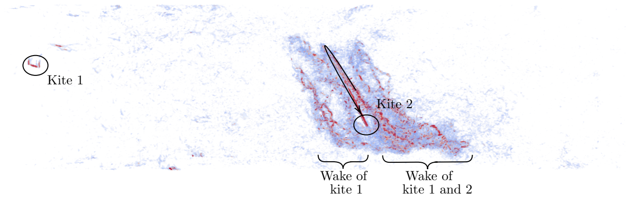
Figure 22. Instantaneous vorticity field volume rendering, at the beginning of a reel out phase of the first kite, for a two-kite configuration where the kites fly out of phase; illustrating the second kite flying in the first kite’s wake.
