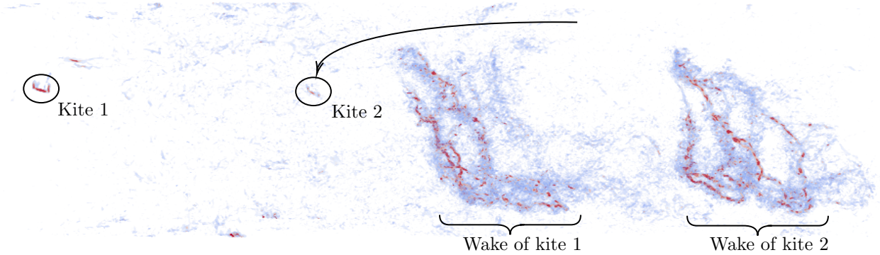
Figure 18. Instantaneous vorticity field volume rendering, at the beginning of a reel out phase, for a two-kite configuration where the kites fly in-phase; illustrating the second kite avoiding the first kite's wake.
