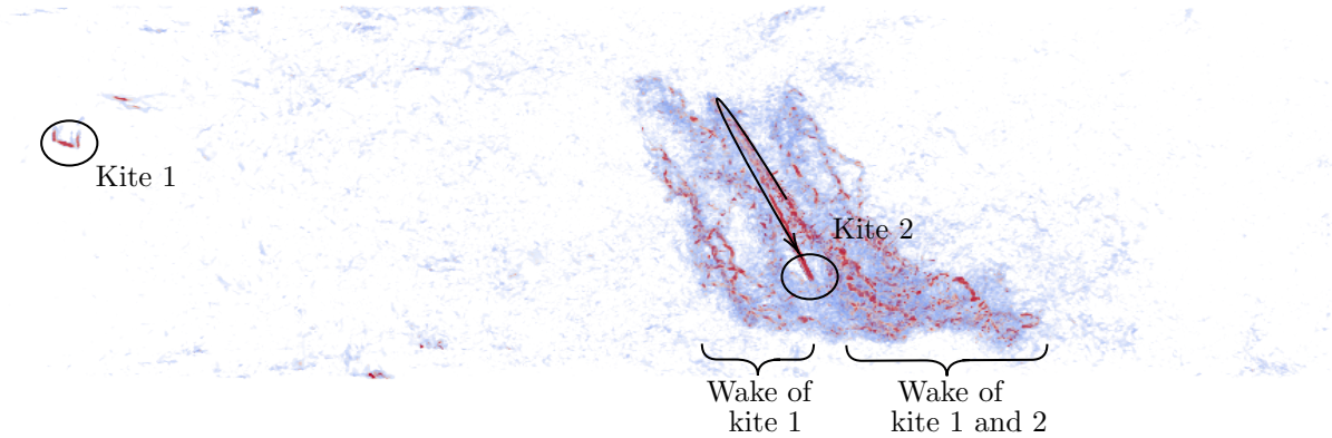
Figure 22. Instantaneous vorticity field volume rendering, at the beginning of a reel-out reel-out phase of the first kite, for a two-kite configuration where the kites fly out of phase; illustrating the second kite flying in the first kite’s wake.
