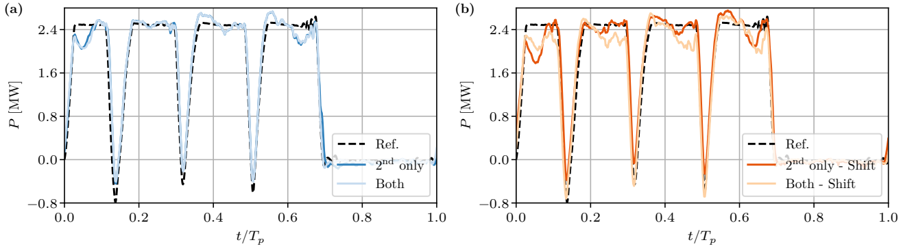
Figure 21. Six-cycle averaged power of the second kite flying in LES with AL in a 6 % TI flow flying the in-phase (a) or phase-shifted (b) trajectory; also compared to a “single” kite.
