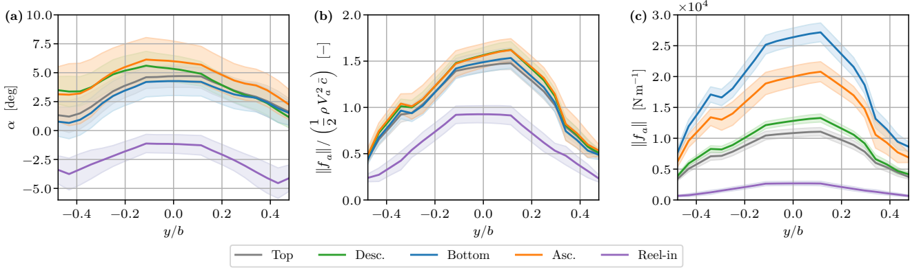
Figure 13. Six-cycle averaged aircraft angle of attack (a) and wing loading, dimensionless (b) and dimensional (c), together with their standard deviation (shaded area), for LES with AL in a 6 % TI flow. They are represented when the kite is at the top and bottom positions, and in the middle of the descending and ascending phases, of the reel-out loops, as well as during the reel-in phase
