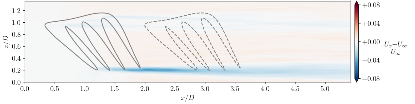
Figure 14. Six-cycle averaged streamwise velocity deficit of a single kite wake in a vertical longitudinal plane at the center of the trajectory. The location of a virtual kite downstream in is indicated by a dashed line.
