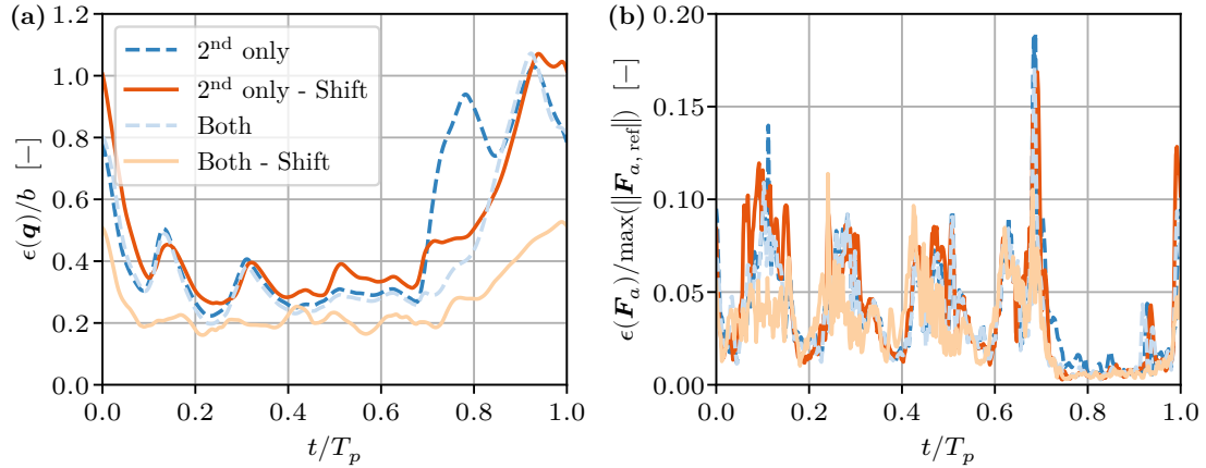
Figure 20. Six-cycle averaged error in position \epsilon(\mathbf{q}) = \text{RMS}(\|\mathbf{q} - \mathbf{q}_{\text{ref}}\|) (a) and forces \epsilon(\mathbf{F}_a) = \text{RMS}(\|\mathbf{F}_a - \mathbf{F}_{a,\text{ref}}\|) (b) for the second kite flying in LES with AL in a 6 % TI flow, the in-phase or phase-shifted trajectory. It is compared to a “single” kite flying at the same place and with the same time delay (i.e., removing the first kite).
