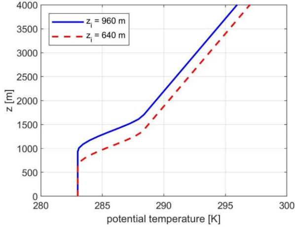
Figure 3: Inflow vertical profiles of potential temperature.
