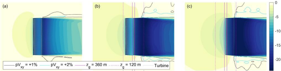
Figure 4: Top view of the percent change in wind speed relative to freestream at hub height for the flat (a), hill windward (b), and hill leeward cases (c). Magenta lines are ground elevation contours; the hill crest is located between the two solid magenta lines.
