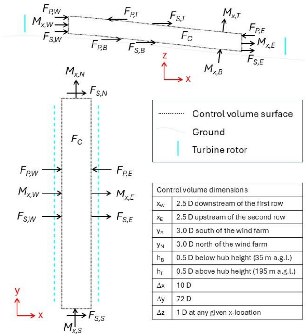
970 Figure A-1: Diagram of the control volume analysis for two-row cases in Section 3.1. The side view, on an xz-plane, is from the hill leeward case.
