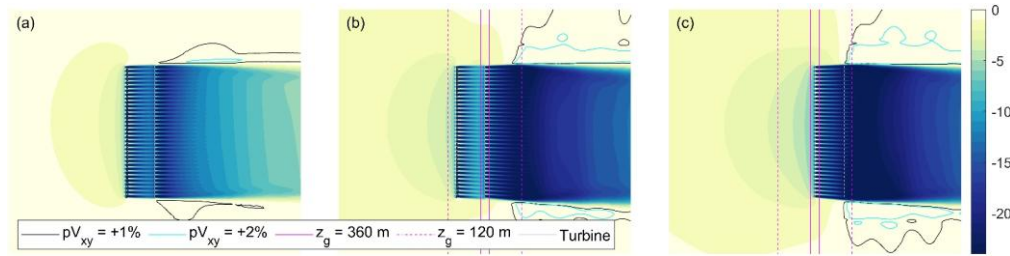
290 Figure 4: Top view of the percent change in wind speed relative to freestream at hub height for the flat (a), hill windward (b), and hill leeward cases (c). Magenta lines are ground elevation contours; the hill crest is located between the two solid magenta lines.
