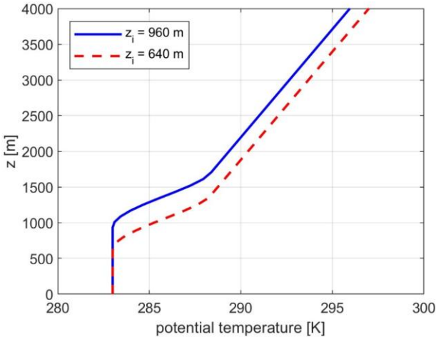
Figure 3: Inflow vertical profiles of potential temperature.
