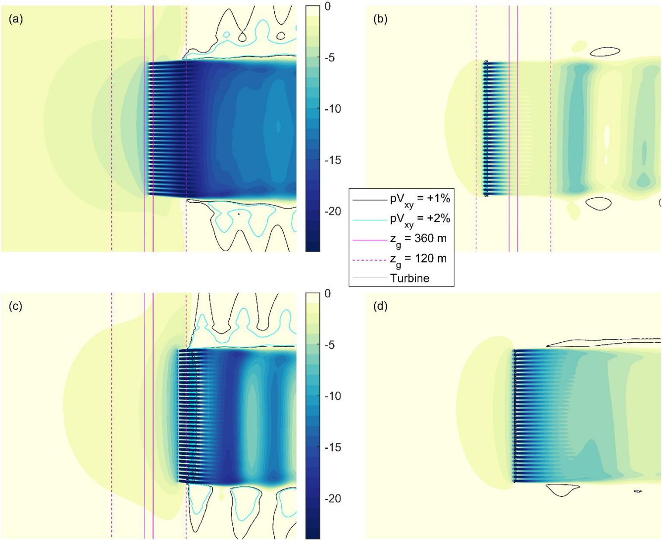
Figure 9: Top view of the percent change in wind speed relative to freestream at hub height for case E (a), case F (b), case G (c), 455 and case H (d) as defined in Table 1. Magenta lines are ground elevation contours; the hill crest is located between the two solid magenta lines.
