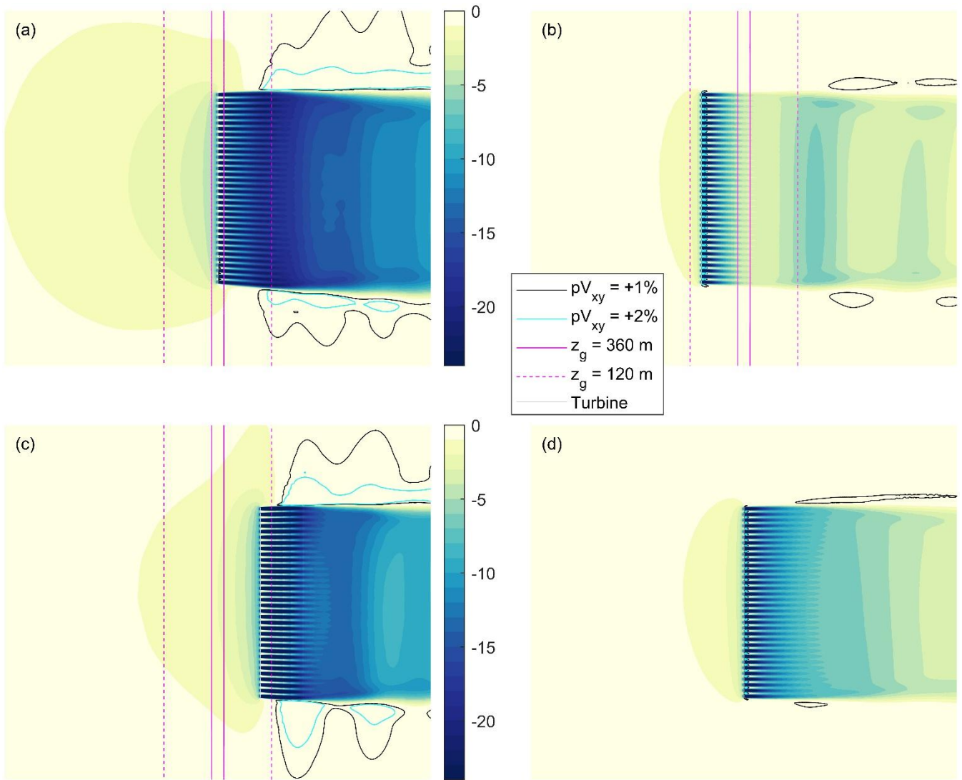
440 Figure 8: Top view of the percent change in wind speed relative to freestream at hub height for Case A (a), Case B (b), Case C (c), and Case D (d) as defined in Table 1. Magenta lines are ground elevation contours; the hill crest is located between the two solid magenta lines.
