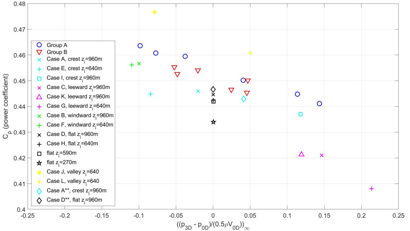
Figure 18: Individual turbine efficiency ( C_p ) vs. freestream pressure coefficient. The pressures are extracted from the freestream simulation at the turbine location and 3 D downstream at hub height at y = 0 m. Power is extracted from isolated turbine simulations. Cases without buoyancy are marked with two asterisks in the legend.
