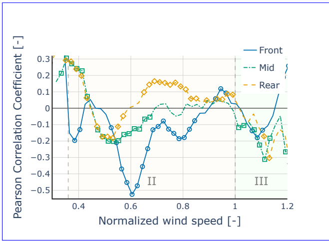
(a) Correlation between wind veer \beta and power deviation PD before REWS correction ( 30^\circ sub-sector).
