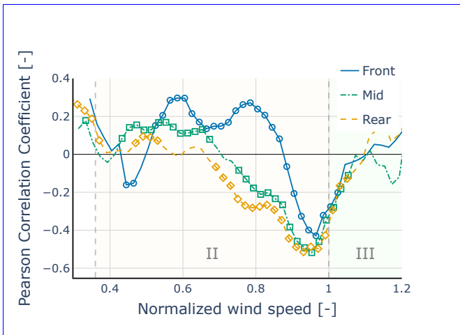
(a) Correlation between TI and power deviation PD using raw TI values ( 30^\circ sub-sector).
