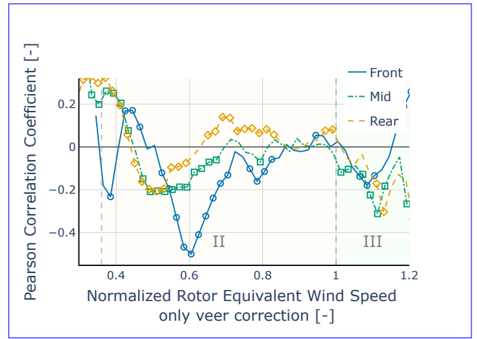
(b) Correlation between wind veer \beta and power deviation PD after REWS (veer-only) correction ( 30^\circ sub-sector).
