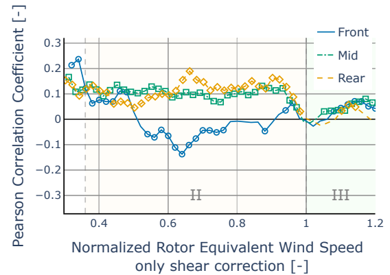
Figure 5. Sliding-window correlation between wind shear \alpha and power deviation PD after REWS (shear-only) correction; changes across the normalized REWS indicate where coupling is reduced or enhanced.
