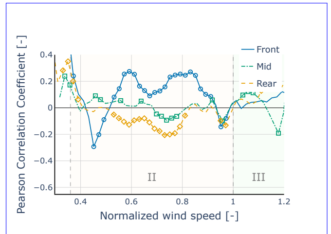
(b) Correlation between TI and power deviation PD using IEC-normalized TI values ( 30^\circ sub-sector).
