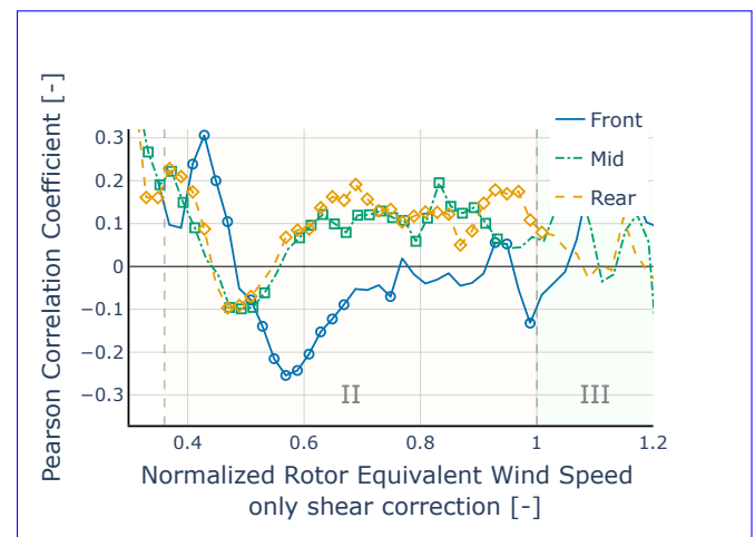
(b) Correlation between wind shear \alpha and power deviation PD after REWS (shear-only) correction (30° sub-sector).
