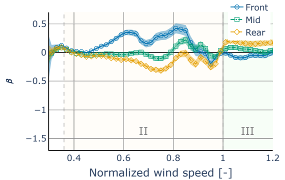
Figure 11. Linear regression slope between TI and normalized active power output deviation at various wind speeds after applying the TI normalization.
