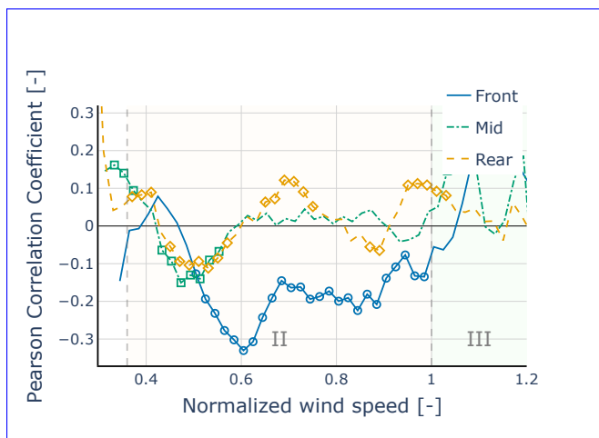
(a) Correlation between wind shear \alpha and power deviation PD before REWS correction (30° sub-sector).
