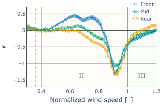
Figure 10. Linear regression slope between TI and normalized active power output deviation at various wind speeds before applying the TI normalization.
