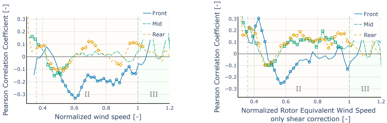
(a) Correlation between wind shear \alpha and active power deviation PD before REWS correction ( 30^\circ sub-sector).
