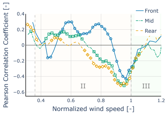
(a) Correlation between TI and power deviation PD using raw TI values ( 30^\circ sub-sector).
