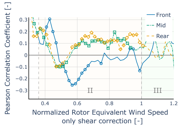
(b) Correlation between wind shear \alpha and power deviation PD after REWS (shear-only) correction ( 30^\circ sub-sector).
