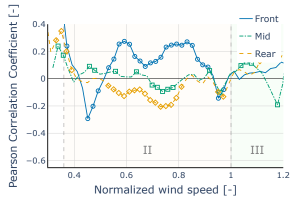
(b) Correlation between TI and power deviation PD using IEC-normalized TI values ( 30^\circ sub-sector).
