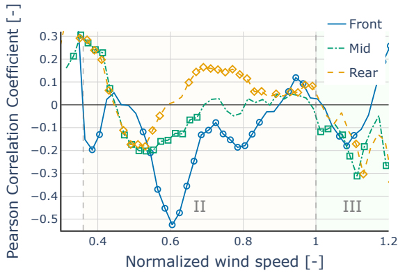
(a) Correlation between wind veer \beta and power deviation PD before REWS correction ( 30^\circ sub-sector).
