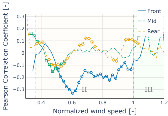
(a) Correlation between wind shear \alpha and power deviation PD before REWS correction ( 30^\circ sub-sector).
