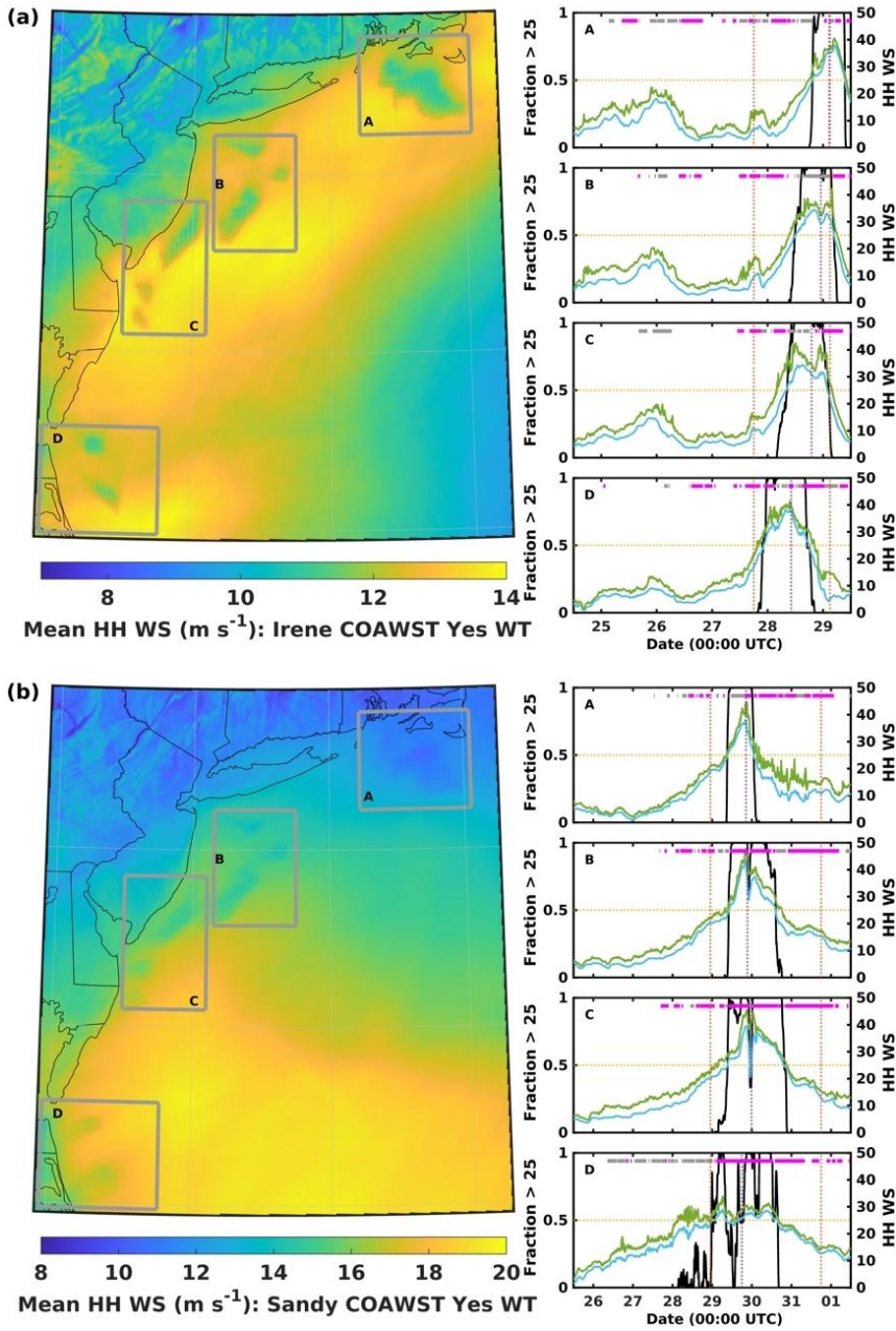
475 Figure 8: Mean simulated hub-height wind speed (HH WS) from COAWST with the wind farm parameterization (WFP) active for (a) Hurricane Irene and (b) Hurricane Sandy. The time series show the fraction of wind turbine (WT) grid cells with HH WS > 25 m s -1 (left axis, black) plus the mean (blue) and maximum (green) HH WS in those grid cells (right axis). Gray (magenta) symbols at the top of the time series indicate times when the mean HH WS from WRF exceeds (is lower than) COAWST by > 0.5 m s -1 . Orange 480 dashed lines indicate the start and end time of storm tracking within d02. The purple dashed line represents the time when the location of the minimum sea level pressure (SLP) is closest to the lease area (LA) cluster center. The yellow line indicates HH WS = 25 m s -1 . See also Figs. S13 and S14.
