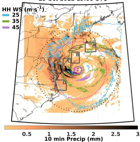
Figure 4: Simulated precipitation from COAWST during two example 10-min periods (background-color) and contours of hub-height wind speed (HH WS) at 25, 35, and 45 m/s for (a) 28 August 2011 09:00 UTC and (b) 29 October 2012 19:00 UTC when the hurricanes are close to wind-turbine (WT) lease areas (LTAs). Magenta rings mark 50-km and 375-km from the minimum sea-level pressure (SLP). The black rings mark the mean outermost radii of 18 m/s WSs at 10 m ( R_{10} ) of (a) 304 km and (b) 541 km. For legibility, the colorbar is truncated. Maximum 10-min precipitation in any grid cell is (a) 13.8 mm and (b) 16.8 mm. Similar output from WRF is shown in Fig. S4.
