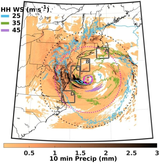
Figure 4: Simulated precipitation from COAWST during two example 10 min periods (background color) and contours of hub-height wind speed (HH WS) at 25, 35, and 45 m s -1 for (a) 28 August 2011 09:00 UTC and (b) 29 October 2012 19:00 UTC when the hurricanes are close to wind turbine (WT) lease areas (LAs). Magenta rings mark 50 km and 375 km from the minimum sea level pressure (SLP). The black rings mark the mean outermost radii of 18 m s -1 WSs at 10 m (R18) of (a) 301 km and (b) 541 km. For legibility, the colorbar is truncated. Maximum 10 min precipitation in any grid cell is (a) 13.8 mm and (b) 16.8 mm. Similar output from WRF is shown in Fig. S4.
