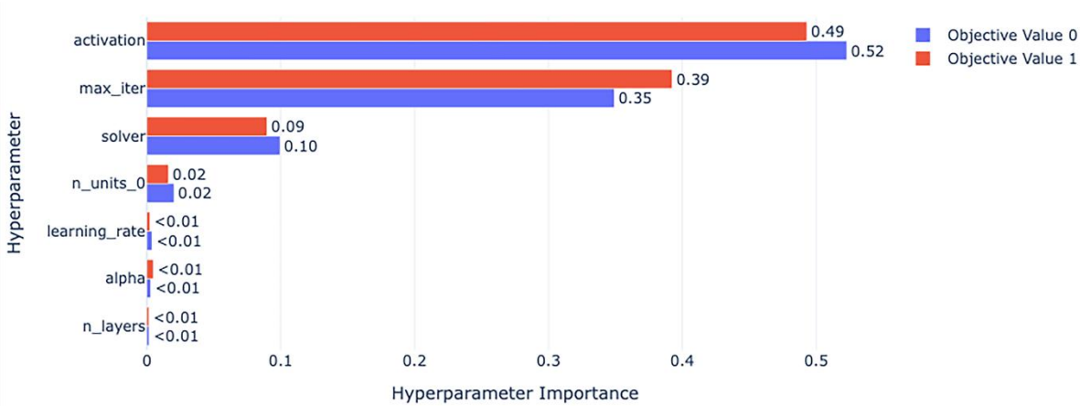
Figure 11: Analysis of hyperparameter significance for local load distribution meta model. (Objective 0: MSE and Objective 1: R^2 )
