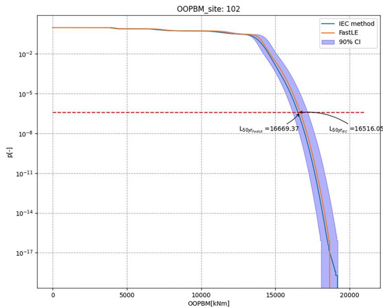
310 Figure 15: Load extrapolation results for test case 102. The blue solid line represents the IEC method, the red line denotes the FastLE method, the shaded area indicates the 90% confidence interval, and the red dashed line corresponds to the probability of 3.8 \times 10^{-7} .
