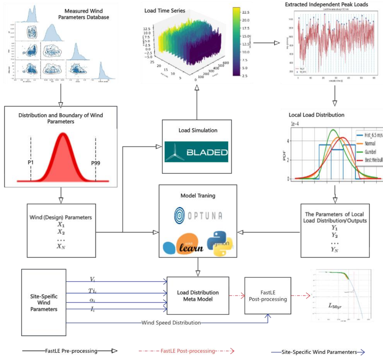
Figure 14: the framework of FastLE . The black solid lines denote pre-processing, the red dashed lines represent post-processing, and the blue solid lines indicate the site-specific application.
