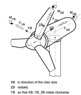
Figure 4: Coordinate system of wind turbine blade
