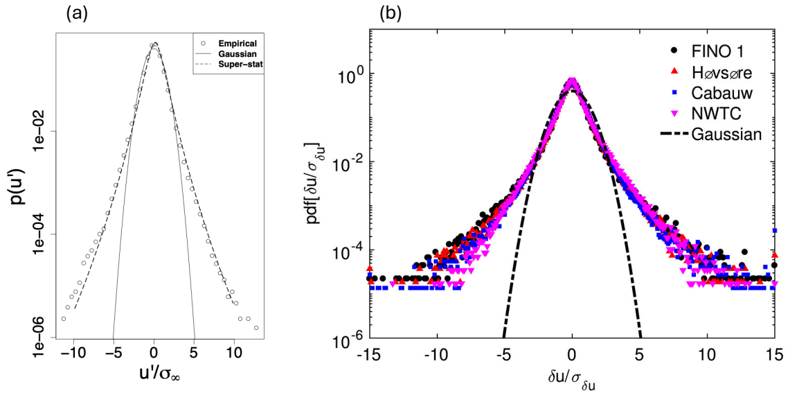
Figure 7. A pdf of fluctuating velocities form FINO1 data of January 2006. The fluctuating quantity \mu is given as u' in units of the standard deviation, Fig. 2 (b) in Morales et al. (2012) reprinted by permission from John Wiley and Sons. Copyright ©2011 John Wiley & Sons, Ltd. (b) A pdf of wind ramps, i.e., time increments, \delta u , from four tall-tower sites (FINO1, Høvsøre, Cabauw, and National Wind Technology Center (NWTC)). Multiyear, 10-min averaged wind data measured by the topmost sensors on these towers are used here (source: DeMarco and Basu, 2018, licensed under CC BY 4.0 license).
