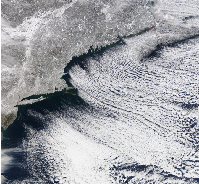
Figure 11. (a) Satellite image of clouds over the East Coast of the United States associated with a cold air outbreak on January 24, 2011 (NASA Worldview Snapshots), indicating the presence of mesoscale convective circulations, convective rolls closer to the coast, and convective cells further downwind from the coast. (b) NOAA's wind lidar (HRDL) captured gravity waves on October 6, 1999, during the CASES-99 field campaign (source: Poulos et al., 2002, ©American Meteorological Society. Used with permission.).
