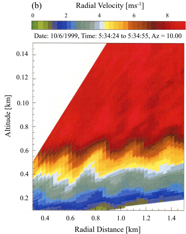
Figure 11. (a) Satellite image of clouds over the East Coast of the United States associated with a cold air outbreak on January 24, 2011 (NASA Worldview Snapshots), indicating the presence of mesoscale convective circulations, convective rolls closer to the coast, and convective cells further downwind from the coast. (b) NOAA's wind lidar (HRDL) captured gravity waves on October 6, 1999, during the CASES-99 field campaign (source: Poulos et al., 2002, ©American Meteorological Society. Used with permission.).
