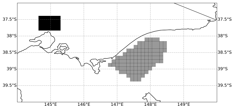
Figure 5. Gridpoints in the BARRA dataset corresponding to the Gippsland offshore priority area (grey) and the Melbourne Metropolitan area (black).
