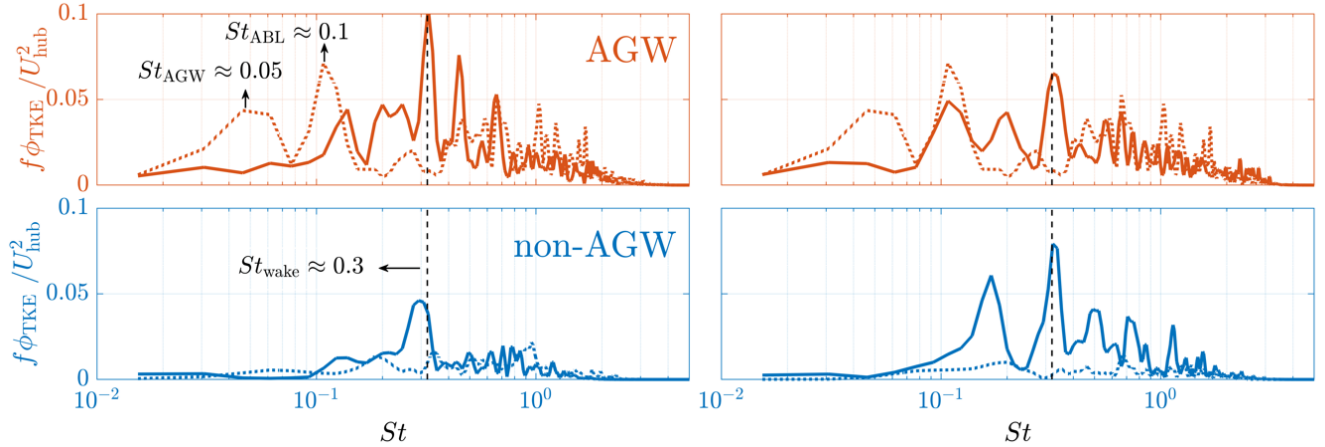
Figure 9. TKE spectra multiplied by the frequency f and non-dimensionalized by U_{\text{hub}}^2 as a function of Strouhal number St = fD/U_{\text{hub}} . The data are compared between the AGW (top) and non-AGW (bottom) cases. The dotted and solid lines represent spectra calculated for the inflow ( (x/D, y/D, z/D) = (-2, 0, 0) ) and wake, respectively. The wake spectra in the left and right panels are 4D and 8D downstream, respectively.
