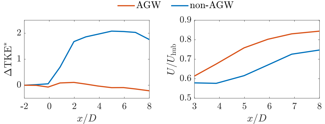
Figure 8. Left: Inflow-normalized TKE generation, \Delta TKE^*_{\text{mean}} , at each streamwise location. Right: Mean streamwise wake deficit along the turbine centerline. The data are compared between the AGW (red line) and non-AGW (blue line) cases.
