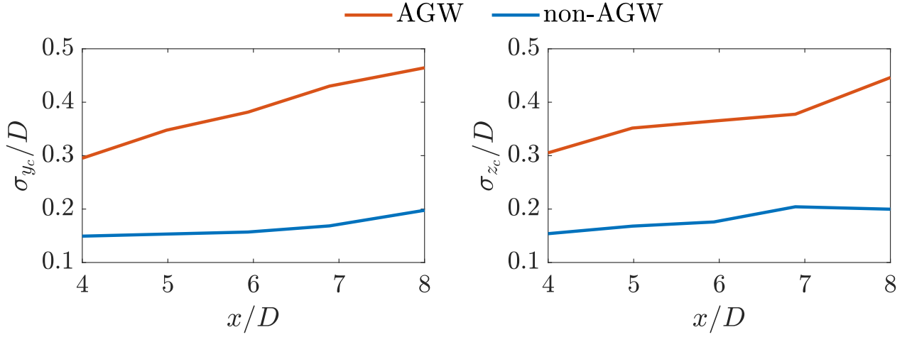
Figure 6. Mean magnitudes of wake meandering in the spanwise (left) and (right) vertical directions for distances 4D - 8D downstream of the turbine. The data are compared between the AGW (red line) and non-AGW (blue line) cases.
