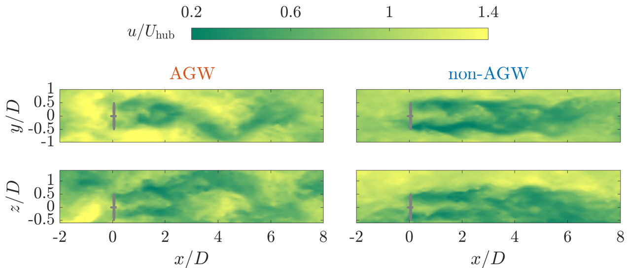
Figure 5. Instantaneous streamwise velocity normalized by U_{\text{hub}} in the spanwise (top) and (bottom) vertical planes passing through the turbine center. The data are compared between the AGW (left) and non-AGW (right) cases. The gray bar in each plot indicates the turbine location.
