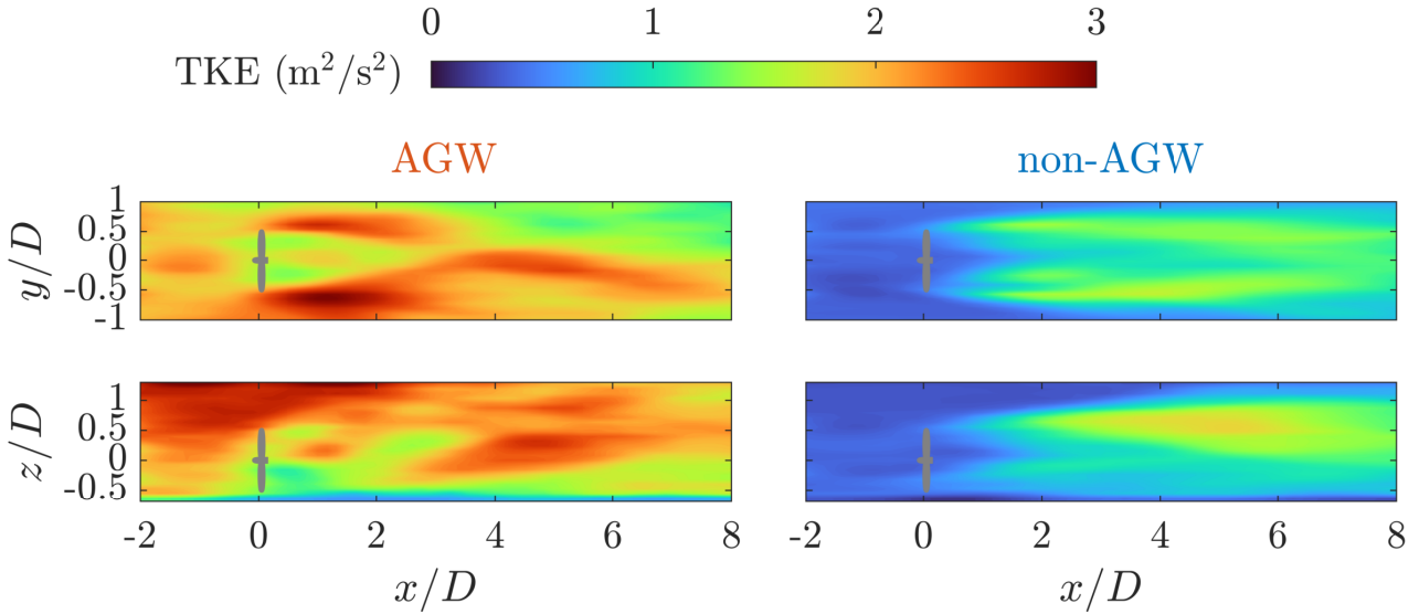
Figure 7. TKE in the spanwise (top) and vertical (bottom) planes passing through the turbine center. The data are compared between AGW (left) and non-AGW (right) cases.
