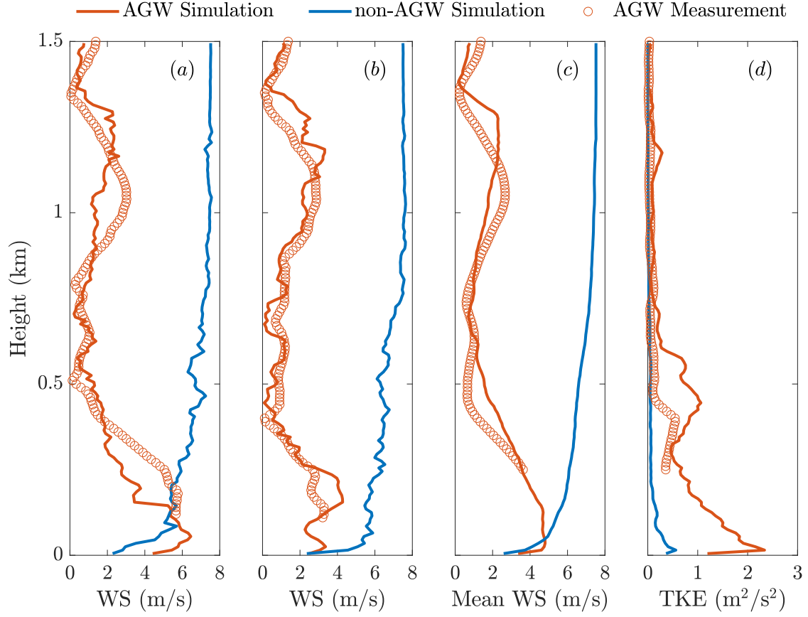
Figure 3. Vertical profiles of (a) instantaneous wind speed at AGW crest, (b) instantaneous wind speed at AGW trough, (c) mean wind speed and (d) turbulent kinetic energy. Data are compared between AGW simulation (red lines), non-AGW simulation (blue lines) and AGW measurement (red circles). The mean wind speed and turbulent kinetic energy at lower heights are not shown for AGW measurement due to the lack of wind-speed data over several time steps, as shown in the top-left contour in Fig. 2.
