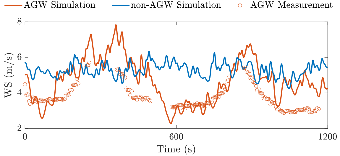
Figure 4. Time series of wind speed at hub-height. Data are compared between AGW simulation (red lines), non-AGW simulation (blue lines) and AGW measurement (red circles).
