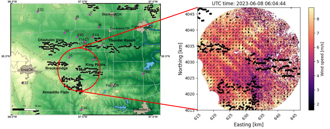
Figure 1. Left: Map of AWAKEN measurement sites. The contour value is elevation over the sea level. The terrain is a fluvial plain with a gradual west-to-east slope (Debnath et al., 2022). This figure is adapted from Moriarty et al. (2024). Right: Radar measurement taken approximately at the hub height during the AGW event on 8 June 2023. The figure is provided by US National Renewable Energy Laboratory (NREL). Black solid circles represent wind turbines.
