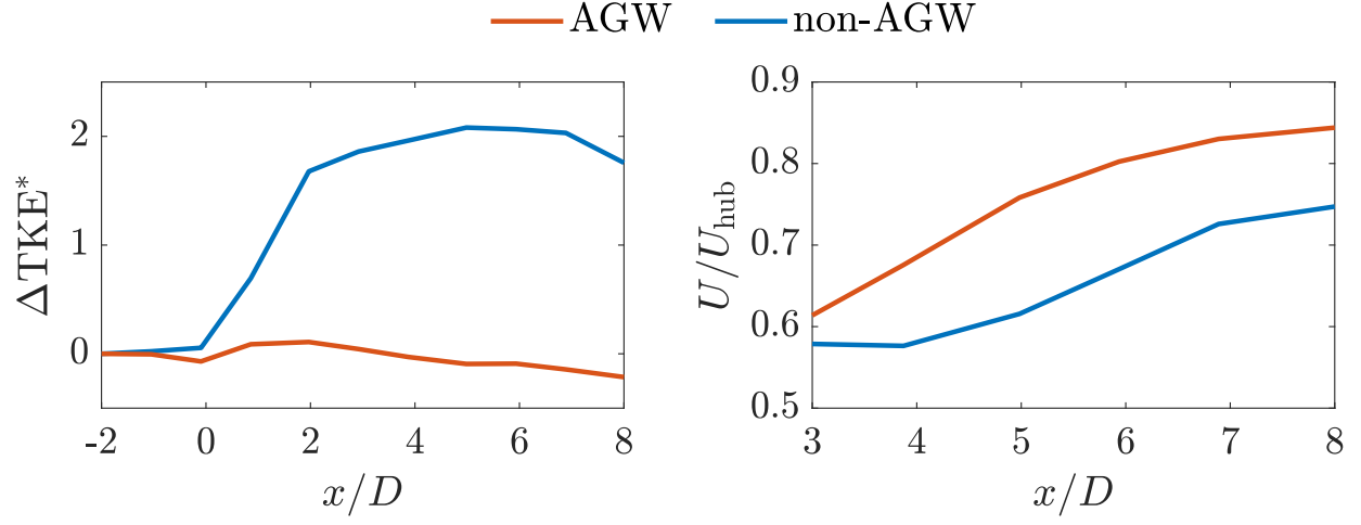
Figure 8. Left: Inflow-normalized TKE generation, \Delta TKE^*_{mean} , at each streamwise location. Right: Mean streamwise wake deficit along the turbine centerline. The data are compared between the AGW (red line) and non-AGW (blue line) cases.
