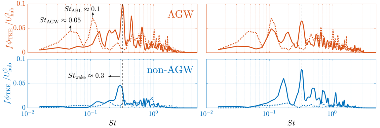
Figure 9. TKE spectra multiplied by the frequency f and non-dimensionalized by U_{hub}^2 as a function of Strouhal number St = fD/U_{hub} . The data are compared between the AGW (top) and non-AGW (bottom) cases. The dotted and solid lines represent spectra calculated for the inflow ( (x/D, y/D, z/D) = (-2, 0, 0) ) and wake, respectively. The wake spectra in the left and right panels are 4D and 8D downstream, respectively.
