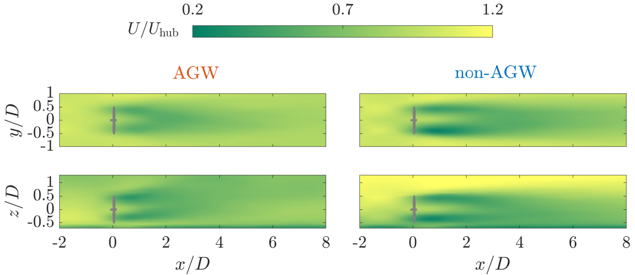
Figure 10. Mean streamwise velocity normalized by U_{\text{hub}} in the spanwise (top) and vertical (bottom) planes passing through the turbine center. The data are compared between AGW (left) and non-AGW (right) cases. The gray bar in each plot indicates the turbine location.
