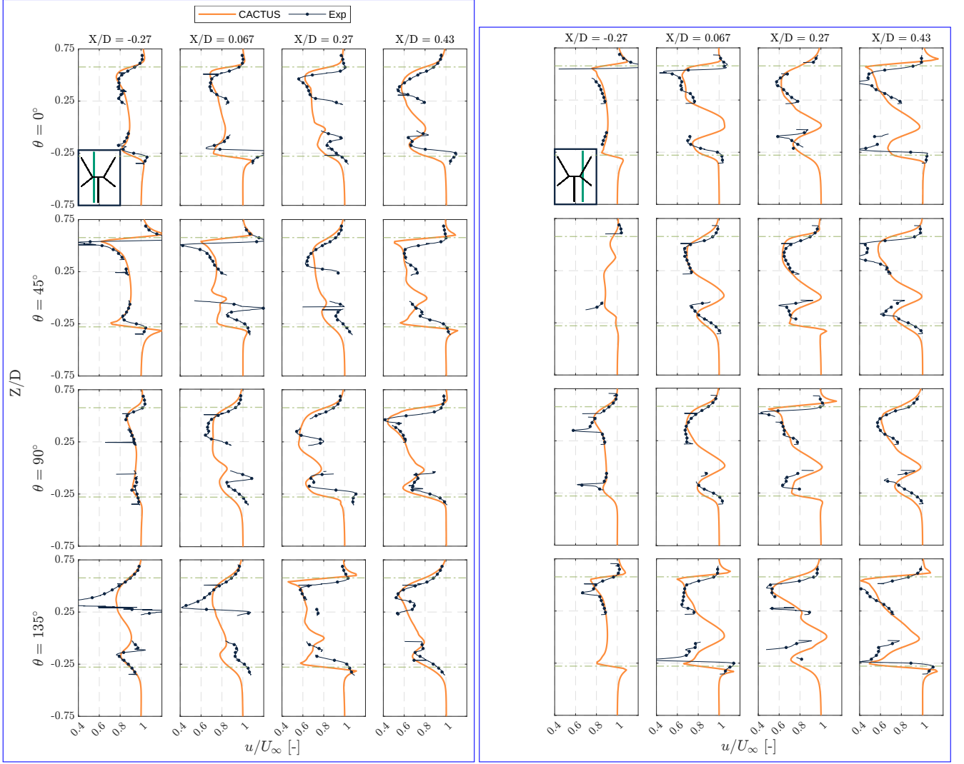
Figure 7. Comparison of the streamwise velocity u/U_\infty slices along the height of the X-Rotor at lateral position Y/D = -0.125 (left) and 0.25 (right) at discrete streamwise locations X/D = [-0.27, 0.067, 0.27, 0.43] at phase locked azimuths \theta = [0^\circ, 45^\circ, 90^\circ, 135^\circ] . The inset figure in the first tile is presented to indicate the location of the slice with respect to the rotor - the green line is the Y/D slice along the height of the rotor.
