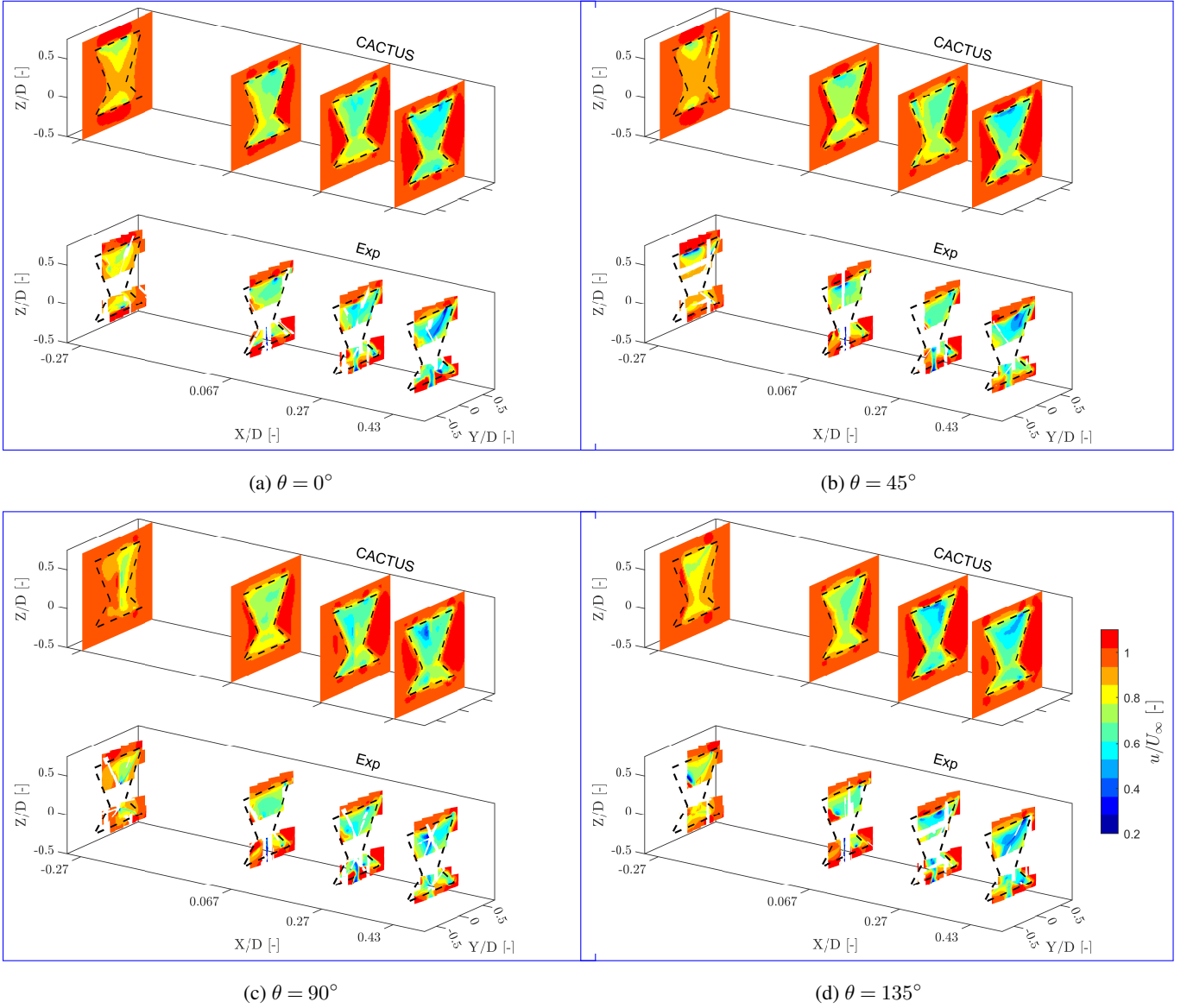
Figure 5. Normalised streamwise velocity ( u/U_\infty ) contours of the X-Rotor at azimuths \theta = [0^\circ, 45^\circ, 90^\circ, 135^\circ] respectively at downstream locations X/D = -0.27, 0.067, 0.27, 0.43 where D is the rotor diameter. The numerical and experimental results are shown in the upper and lower tile respectively. The black dash lines indicate the projected frontal area of the rotor on the corresponding plane. The x-axis is magnified to enhance visibility.
