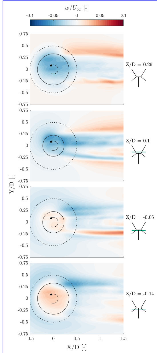
Figure 12. Time-averaged vertical component of the velocity field of the rotor at sections along the height of the rotor at Z/D = 0.29, 0.1, -0.05 , and -0.14 as viewed from the top. The inset figure shows the locations of the planes along the height of the X-Rotor graphically. The dashed black line indicates the tip-diameter of the X-Rotor and the solid black line indicates the local diameter corresponding to the height. Red indicates upwash (out of the plane) and blue indicates downwash (into the plane).
