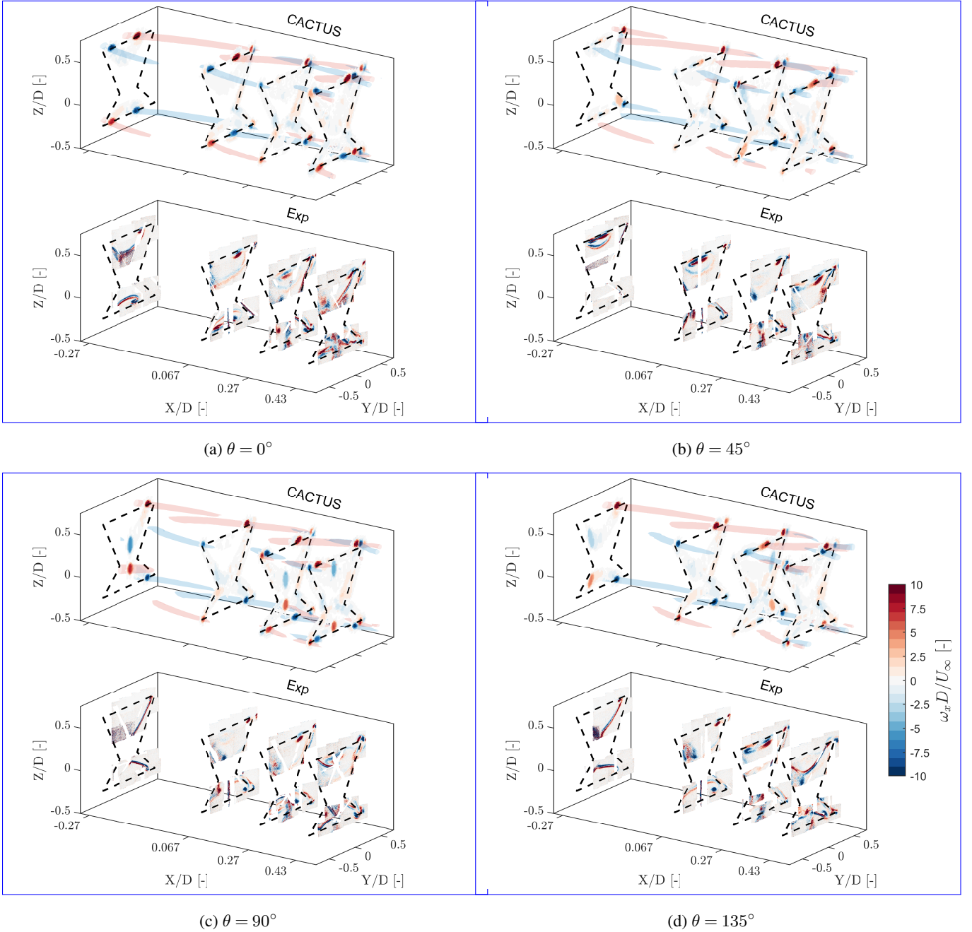
Figure 6. Normalised streamwise vorticity ( \omega_x D/U_\infty ) contours of the X-Rotor at azimuths \theta = [0^\circ, 45^\circ, 90^\circ, 135^\circ] respectively at downstream locations X/D = -0.27, 0.067, 0.27, 0.43 where D is the rotor diameter. The numerical for CACTUS (top) and experimental results are shown in the upper and lower tile respectively experiments (bottom). Isosurfaces generated from the CACTUS simulations isosurfaces are overlayed over it to show the evolution of the vortices and represent vortices with non-dimensionalised strength of 6 and above. The black dash lines indicate the projected frontal area of the rotor on the corresponding plane. Very low values of vorticity are hidden and x-axis is magnified to enhance visibility.
