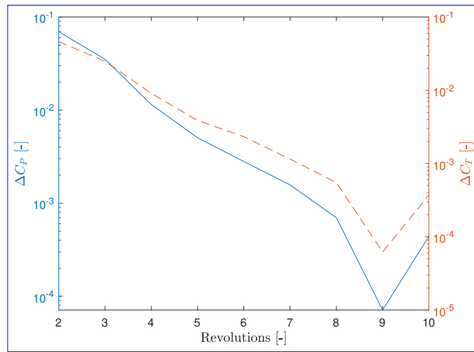
Figure A4. Convergence plot of power and thrust. The Y-axes are in logarithmic scale
