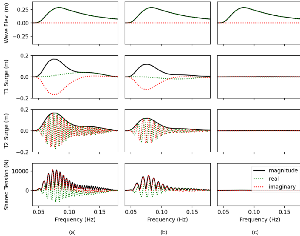
Figure 14. Complex response amplitudes predicted by RAFT for (a) 0^\circ (b) 45^\circ and (c) 90^\circ wave headings
