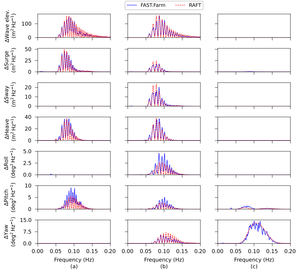
Figure 13. PSDs of relative wave elevation and relative motions between T1 and T2 obtained with RAFT and FAST.Farm for (a) 0^\circ , (b) 45^\circ , and (c) 90^\circ wind and wave headings
