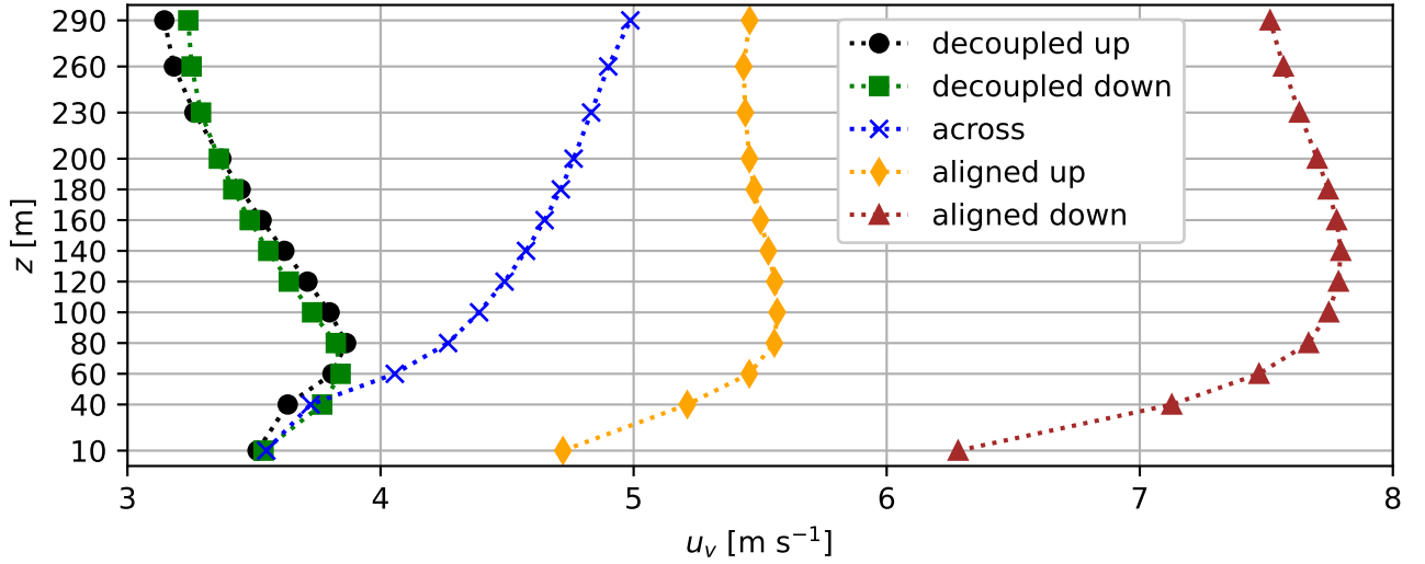
Figure 3. Average observational wind speed profiles by WR. Only complete profiles (without gaps at any heights) are included
