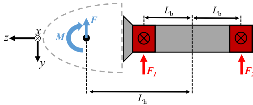
Figure 2. Force diagram of a main shaft in a four-point support drivetrain. Note, the z -axis is aligned with the turbine drivetrain and hence sits at a tilt angle relative to the ground. Force and moment vector components (including the definition of “positive direction”) at each location are defined via the depicted HAWC2 reference frame.
