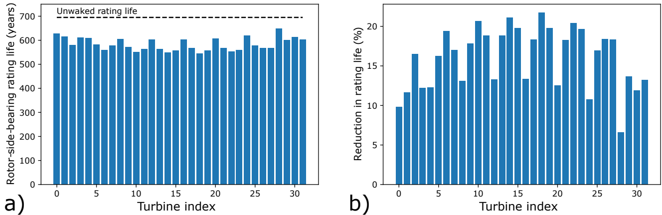
Figure 6. a) Rating life results for all rotor-side main bearings, obtained from a wind direction rose with parameters \alpha = 0.7 and f = 0.35 . The rating life corresponding to unwaked operation is also shown. b) Percentage reductions in rotor-side main bearing rating lives, for the same wind rose, relative to the unwaked rating life.
