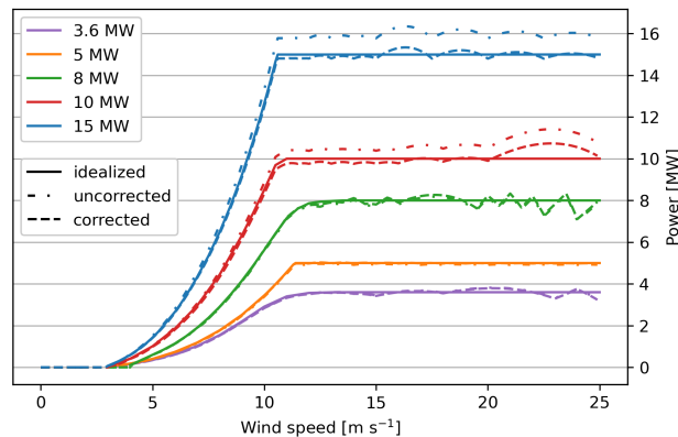
Figure 1. Power curves for different turbines. Idealized power (solid lines), uncorrected curves using turbine-NRELturbine power coefficients (dashed-dotted lines), and corrected curves (dashed lines).
