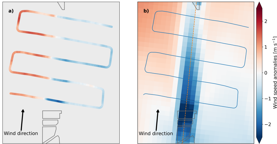
Figure 5. Anomalies for wind Wind speed anomalies, calculated as deviations from the respective dataset means, for airborne observations (left) and simulated data from the 3.6 MW scenario simulation (right) in the downstream area of the wind farm cluster Amrumbank West, Meerwind Süd/Ost, and Nordsee Ost and the Butendiek wind farm in the north (in solid gray) on the 10 September 2016 at 09:00 UTC. The red dashed line marks the cross-section depicted in Fig. 6.
