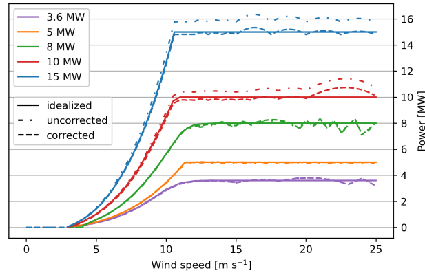
Figure 1. Power curves for turbines with different rated capacities. Idealized power (solid lines), uncorrected curves calculated directly from the provided turbine power coefficients (dashed-dotted lines), and corrected curves obtained following the application of the scale factor (dashed lines).
