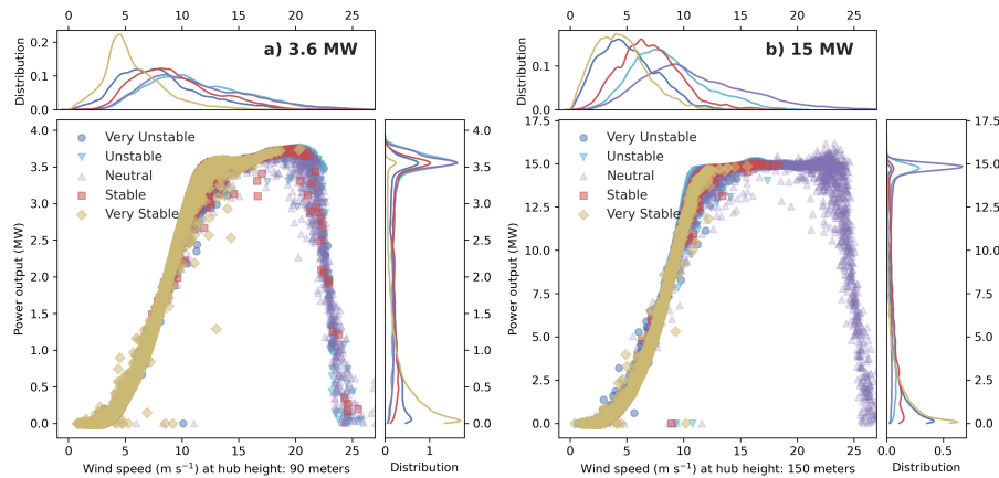
Figure 8. Model simulated power curves based on hourly averaged data from 3.6 MW (a) and 15 MW (b) turbine types in the period from 2008 to 2018. The power output is classified by atmospheric stability conditions (in colors, plotted from very unstable to very stable, which causes overlaying symbols). Statistical distributions for the power output and wind speed are additionally depicted in the respective figure axes.
