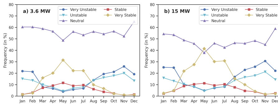
Figure 9. Yearly cycle of occurrences for different atmospheric conditions at the Amrumbank West wind farm in the simulations: a) at 90 meter height for the 3.6 MW scenario, and b) at 150 meter height for the 15 MW scenario in the period from 2008 to 2018.
