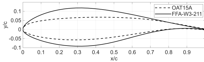
Figure 1. Comparison of the OAT 15A supercritical airfoil (dotted line) and the FFA-W3-211 wind turbine airfoil (solid line).
