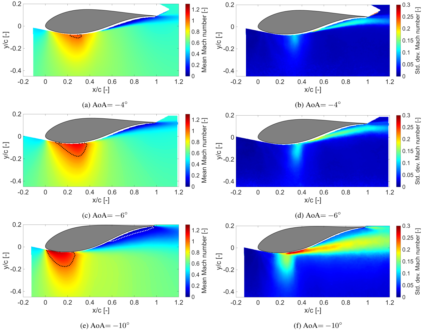
Figure 7. Contours of Mach number: mean values (left column) and standard deviation (right column) for \text{Ma}_\infty = 0.6 . The dotted black line represents a local Mach number of 1. The dotted white line indicates zero streamwise ( x ) velocity.
