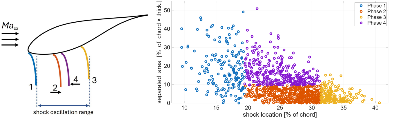
Figure 16. Definition of phases (left) and shock locations versus separated areas during various phases for Ma_\infty = 0.6 , AoA = -10^\circ .
