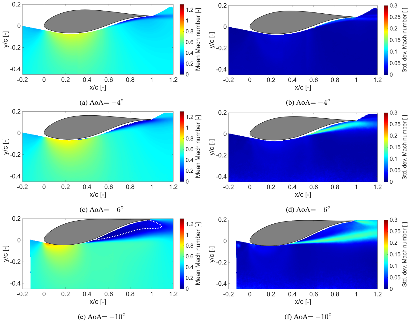
Figure 6. Contours of Mach number: mean values (left column) and standard deviation (right column) for \text{Ma}_\infty = 0.5 . The white dotted line shows zero streamwise (x) velocity.
