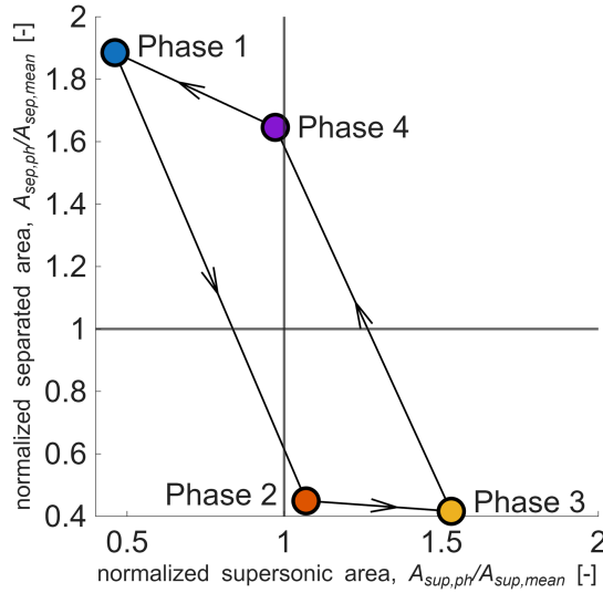
Figure 18. Representation of the transonic buffet cycle in terms of phase-averaged supersonic area ( A_{sup,ph} , along x-axis) and separated area ( A_{sep,ph} , along y-axis), each normalized with the corresponding area in the mean flow for Ma_\infty = 0.6 , AoA = -10^\circ . The areas occupied in the mean flow by supersonic flow ( A_{sup,mean} ) and separated flow ( A_{sep,mean} ) are denoted by solid black vertical and horizontal lines, respectively.
