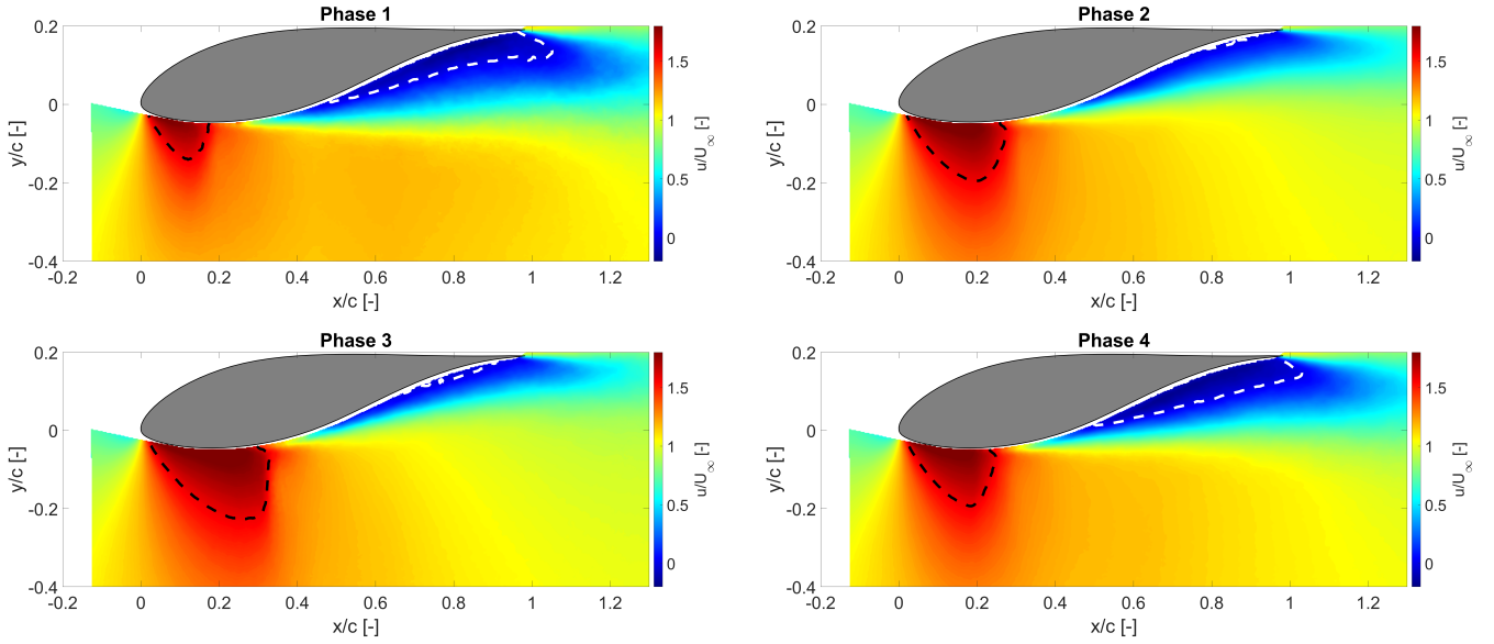
Figure 17. Phase-averaged normalized streamwise velocities for Ma_\infty = 0.6 , AoA = -10^\circ . The dashed black lines enclose the local supersonic region, and the white dashed lines enclose the separated flow.
