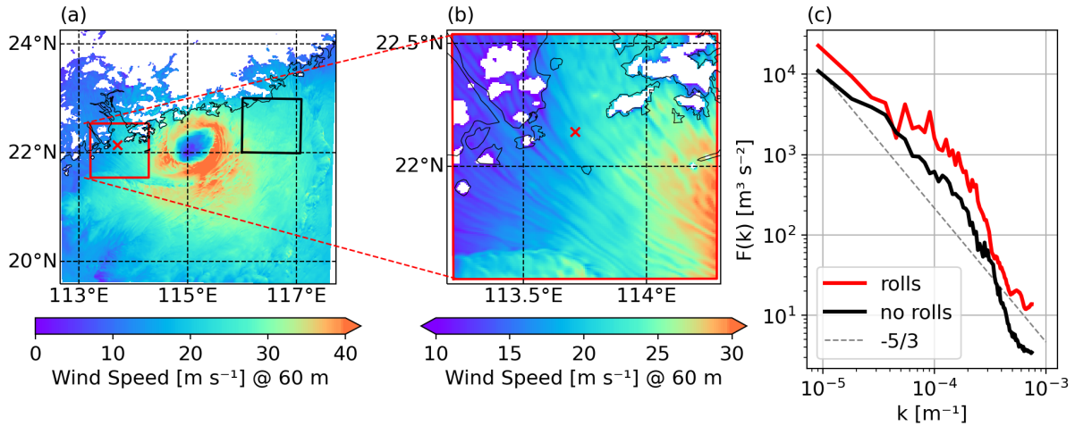
Figure 11. a,b) Simulated horizontal wind speed during typhoon Nuri at 60 m above sea level. Panel b shows a detailed view of the area marked in red in panel a; note the different color scales. The red cross in a and b gives the measurement location, and the black contours give the coastlines. White areas have a terrain elevation larger than 60 m. c) Wind speed power spectra calculated from the simulated wind speed at 60 m from the areas marked in red and black in panel a, representing areas with and without boundary layer rolls. The dashed line gives a slope of -5/3 for reference.
