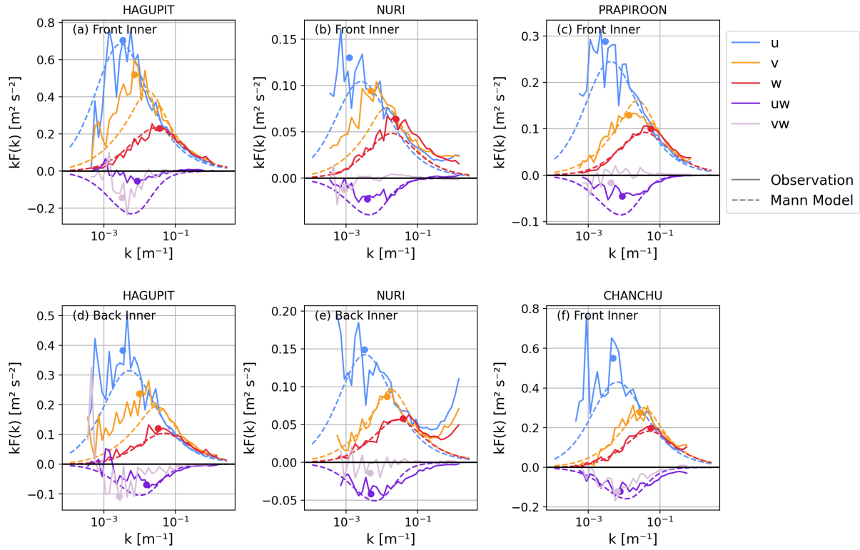
Figure 9. Spectra from the front and back inner cyclone regions of the four typhoon cases : Median of observed spectra (Solid lines), fitted Mann Model (dashed lines), and estimated maxima of the observed spectra (points).
