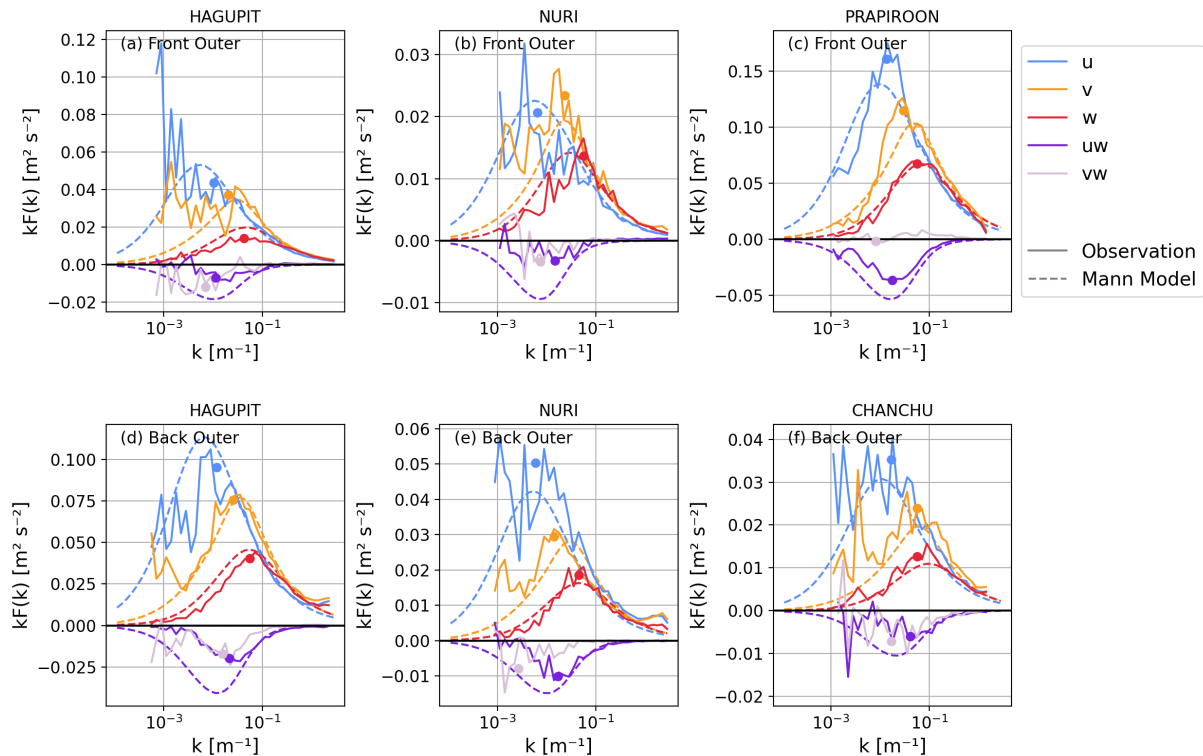
Figure 8. Spectra from the front and back outer cyclone regions of the four typhoon cases cases : Median of observed spectra (Solid lines), fitted Mann Model model (dashed lines), and estimated maxima of the observed spectra (points).
