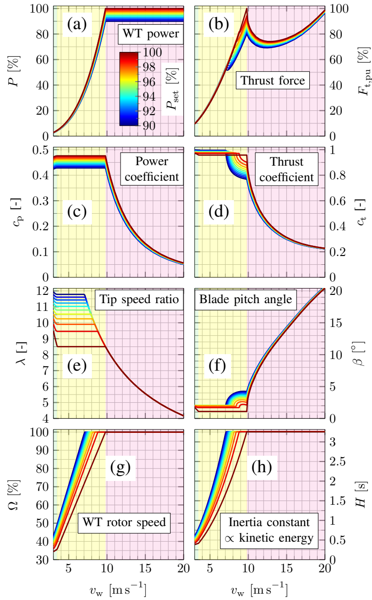
Figure 8. WT steady-state conditions as functions of wind speed v_w for MRS-based derating with power setpoint P_{set} (see steady state calculation in Appendix ??I ).
