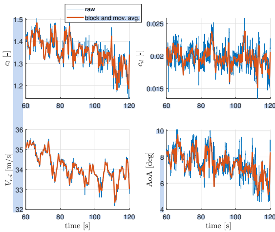
(a) Exemplary time traces of calculated variables over 60 s with and without block and moving average
