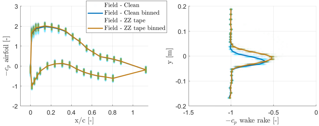
Figure 11. Exemplary results of c_p distributions and wake deficits for the airfoil with and without zig-zag tape
