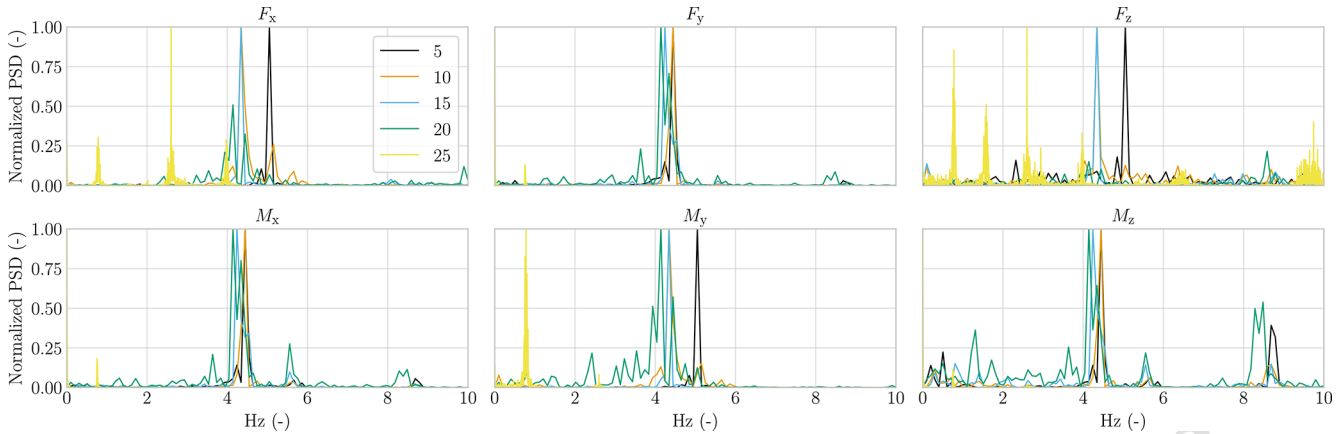
Figure E3. Raw measurements transformed into PSD using FFT and a periodogram function and displayed for the three force and moment components up to 10 Hz. 40
