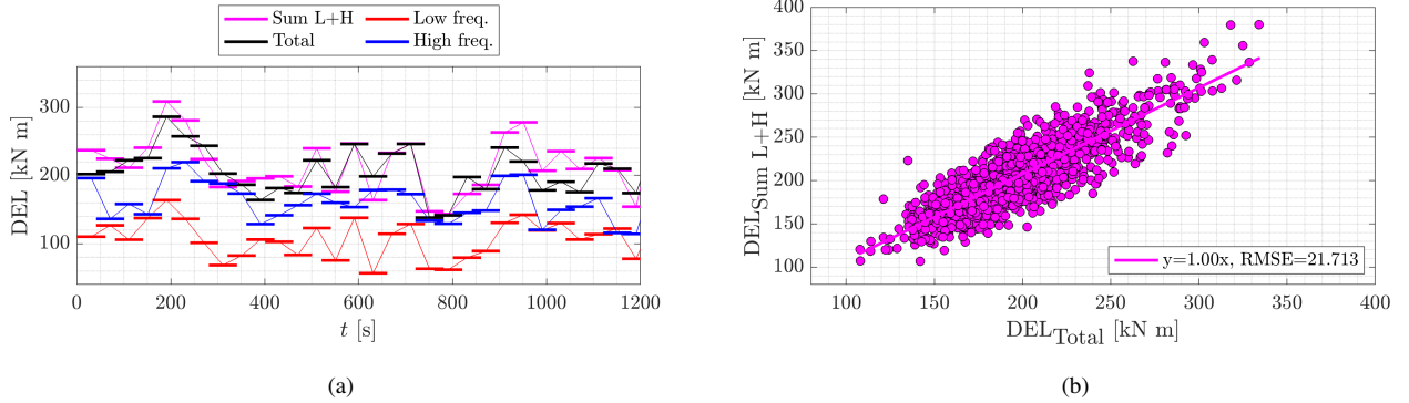
Figure B1. (a) 20-min excerpt of the DELs for the T_{titt} signals at the main shaft. The length of the individual horizontal bars depicts the periods T . (b) Correlation plot between the total load and the sum of the DELs from the low- and high-frequency signals. The DELs are calculated with m = 10 over periods of T = 60 s with an overlap of 30s between periods. The load signals are those calculated from BEM simulations of the 5MW NREL WT with Kaimal fields, with \bar{u} = 7 m/s (see Sec. 3).
