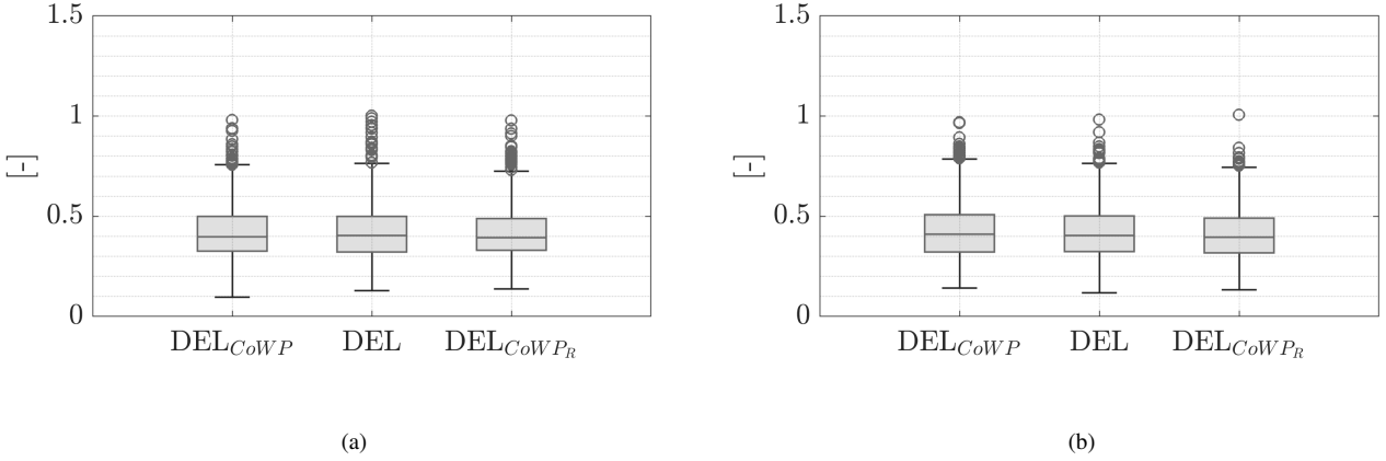
Figure 13. Box plots of the DEL_{CoWP} , DEL , and DEL_{CoWP_R} from normalized and filtered signals of (a) CoWP_y , T_{yaw} , and CoWP_{R,y} , and (b) CoWP_z and T_{tilt} , and CoWP_{R,z} . The DELs are calculated over periods T = 60 s with 30 s of overlapping and with a coefficient m = 10 . The lines defining each box show the median, and the bottom and top edges indicate the 25th ( P_{25} ) and 75th ( P_{75} ) percentiles. The whiskers indicate the most extreme data points. They are calculates as P_{25} - (1.5 \times IQR) and P_{75} + (1.5 \times IQR) . The markers show outliers.
