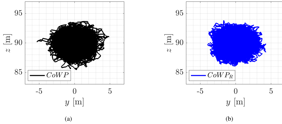
Figure 10. Trajectories on the y - z plane of (a) the original CoWP calculated from the Kaimal data, and (b) the stochastically reconstructed signal \text{CoWP}_R . Intentionally, the data of both CoWP and \text{CoWP}_R for plotting the trajectories in (a) and (b) are not normalized.
