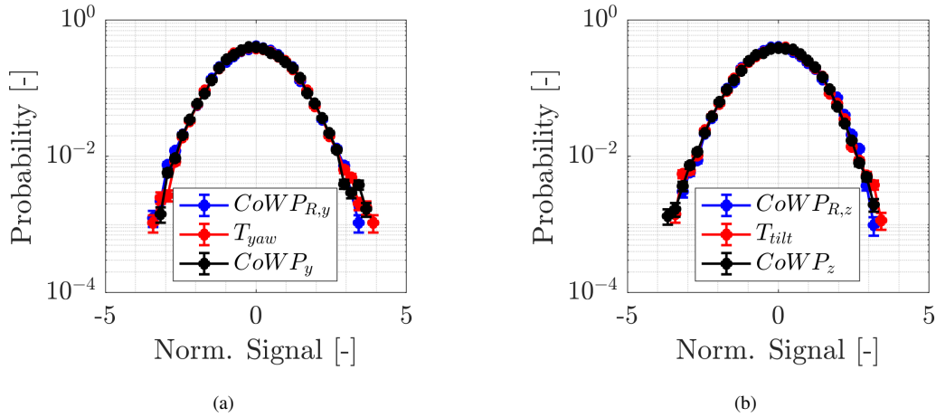
Figure 11. PDF of the CoWP, \text{CoWP}_R and bending moments T . (a) \text{CoWP}_{R,y} , \text{CoWP}_y , and T_{yaw} . (b) \text{CoWP}_{R,z} , \text{CoWP}_z , and T_{tilt} . The signals are normalized and low-pass filtered.
