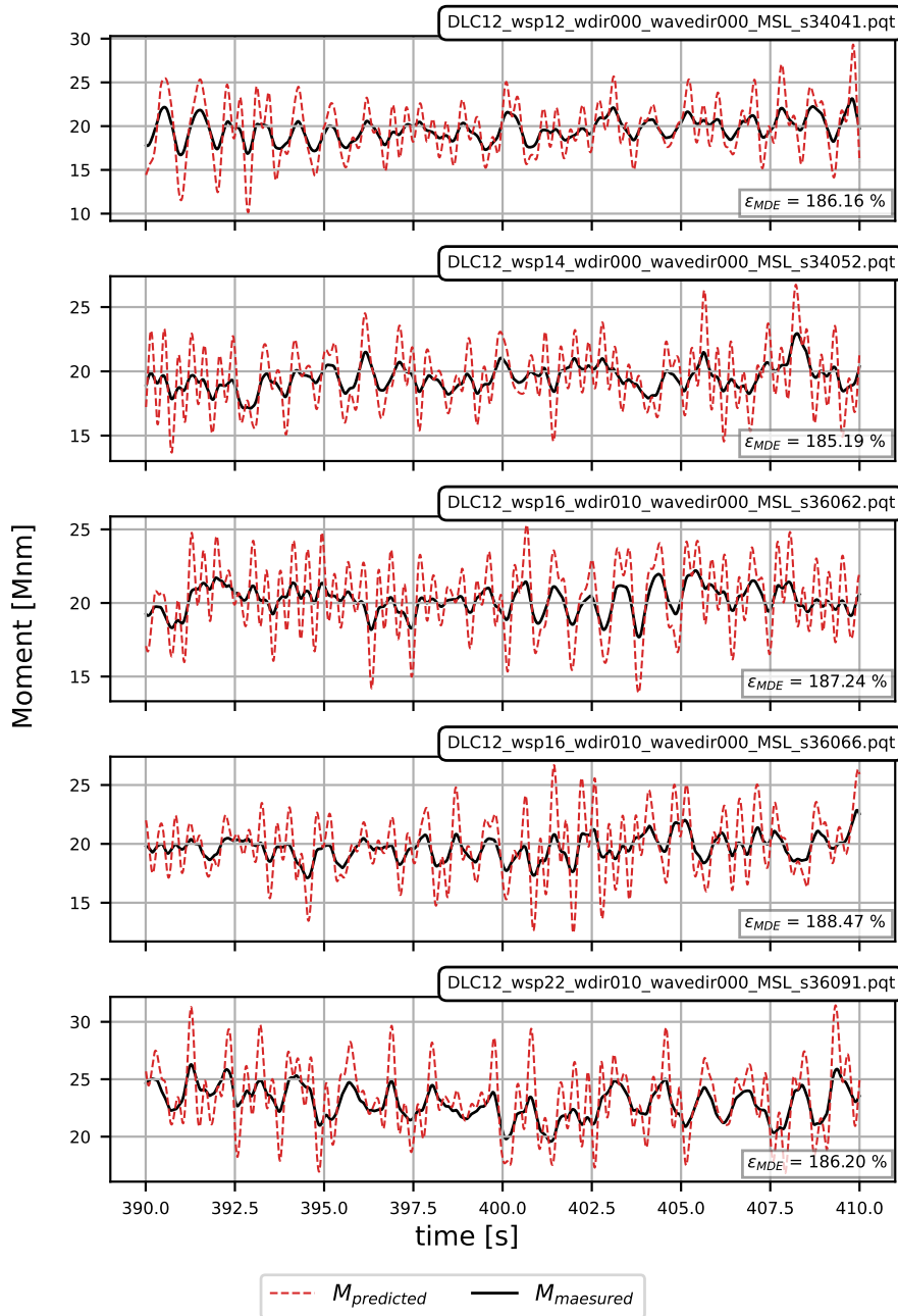
Figure C2. Time-series segments of five representative simulations from DLC 1.2, demonstrating poor MDE performance for the section-selected SS moment histories corresponding to the largest relative MDE errors ( \epsilon_{MDE} ) at a +144 m elevation above the Mean-Sea-Level in the FA direction MSL for DLC 1.2. The time series segments include: 1) the predicted moment history (red) and 2) the true (or measured) moment history (black). PSDs of the moment time-history and the MDE error are presented in Figure ??.
