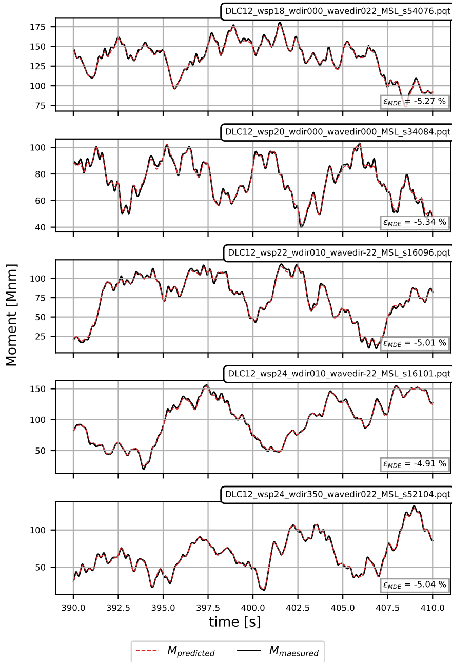
Figure C6. Time-series segments of five representative simulations from DLC 1.2, demonstrating poor MDE performance for the section-selected FA moment histories corresponding to the largest relative MDE errors ( \epsilon_{MDE} ) at the Mean Sea Level in the FA direction elevation 0 m above MSL for DLC 1.2. The time series segments include: 1) the predicted moment history (red) and 2) the true (or measured) moment history (black). PSDs of the moment time history and the MDE error are presented in Figure ??.
