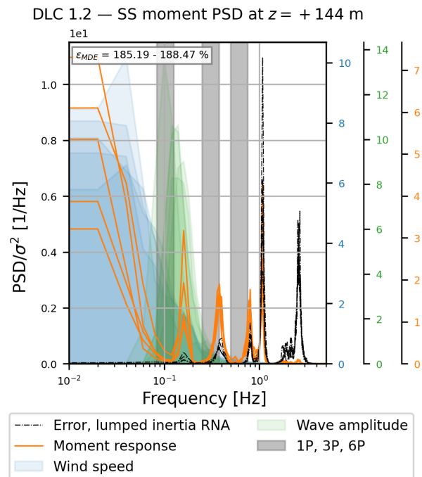
Figure 16. Normalised PSDs representing the MDE performance for the SS moment at the elevation 144 m for five selected moment histories in DLC 1.2. The corresponding selected moment histories are presented in Figure C2. The PSDs include: 1) the MDE error for the lumped inertia RNA model (black), 2) the 10-minute section moment time series (orange), 3) the wind speed in the FA direction (light blue), and 4) the wave amplitude (green). The grey bands indicate the 1P, 3P, and 6P excitation frequencies.
