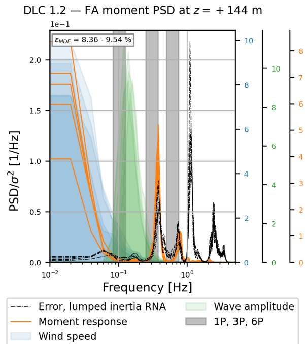
Figure 15. Normalised PSDs representing the MDE performance for the FA moment at the elevation 144 m for five selected moment histories in DLC 1.2. The corresponding selected moment histories are presented in Figure C1. The PSDs include: 1) the MDE error for the lumped inertia RNA model (black), 2) the 10-minute section moment time series (orange), 3) the wind speed in the FA direction (light blue), and 4) the wave amplitude (green). The grey bands indicate the 1P, 3P, and 6P excitation frequencies.
