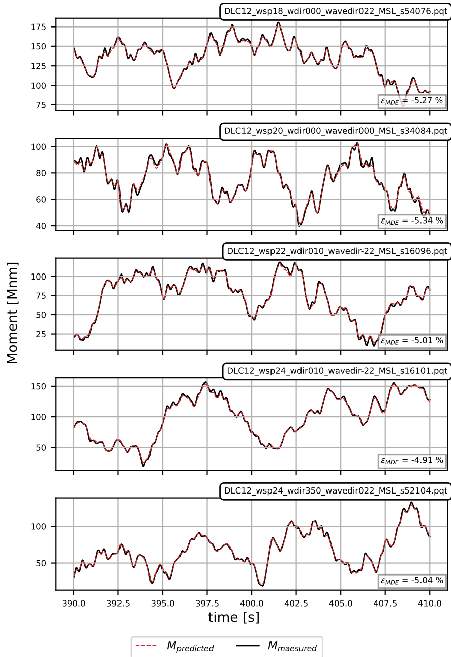
Figure C6. Segments of selected FA moment histories corresponding to the largest relative MDE errors ( \epsilon_{MDE} ) at the elevation 0 m above MSL for DLC 1.2. The time series segments include: 1) the predicted moment history (red) and 2) the true (or measured) moment history (black).
