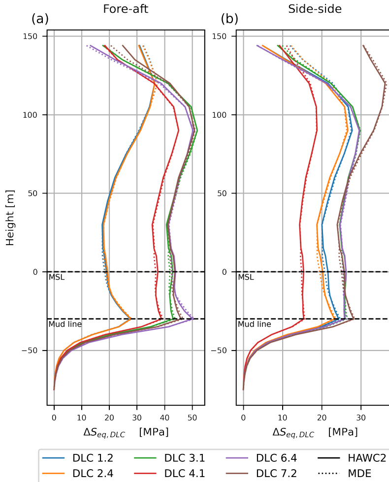
Figure 13. DESs calculated for the individual DLCs based on section moment load histories from HAWC2 (—) and MDE prediction (⋯⋯⋯) in the FA (a) and SS (b) direction of the IEA 15-MW RWT, as presented in (29).
