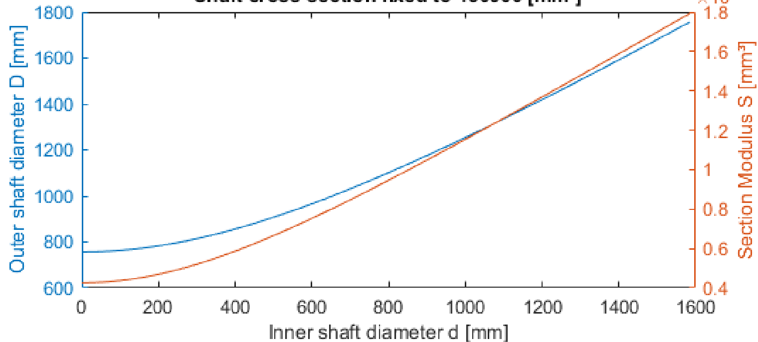
Shaft cross-section fixed to 450000 [mm 2 ]
