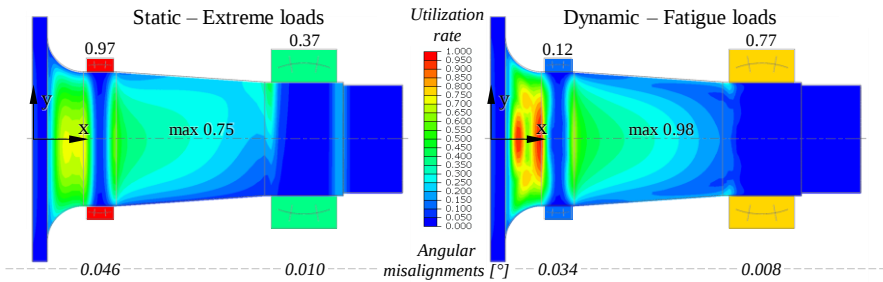
Figure 5: Utilization rates of the cast rotor shaft (FEA), main bearings (DIN EN ISO 76 / 281) and angular shaft misalignment (FEA).
