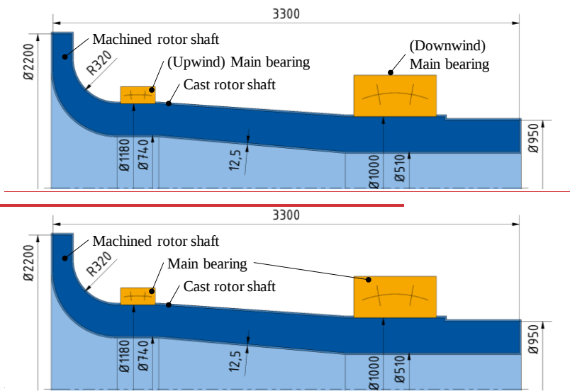
Figure 3: Sketch of the cast rotor shaft and its casting geometry, together with the chosen main bearings.
