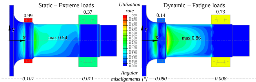
Figure 4: Utilization rates of the hollow forged rotor shaft (FEA), main bearings (DIN EN ISO 76 / 281) and angular shaft misalignment (FEA).
