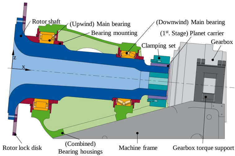
95 Figure 1: Sketch of the maxcap141 MBU in a half section view and adjacent components in full view.
