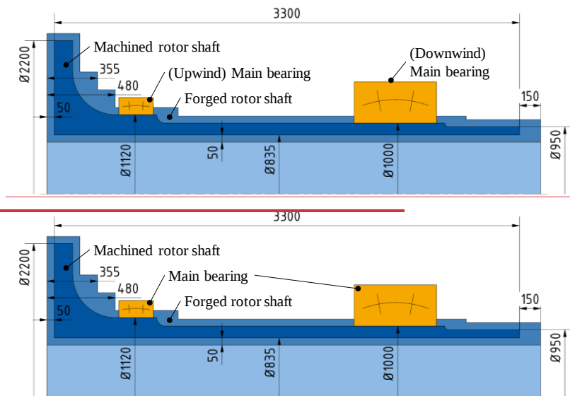
Figure 2: Sketch of the hollow forged rotor shaft and its forging geometry, together with the chosen main bearings.
