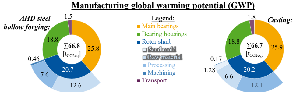
Figure 6: Case study summary: comparison of power density, manufacturing costs and manufacturing GWP of MBUs with cast and AHD steel hollow forged rotor shafts
