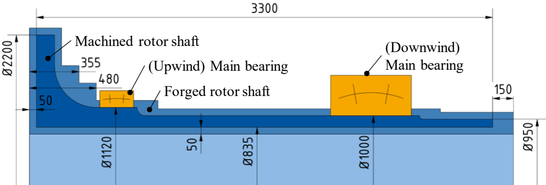
Figure 2: Sketch of the hollow forged rotor shaft and its forging geometry, together with the chosen main bearings.
