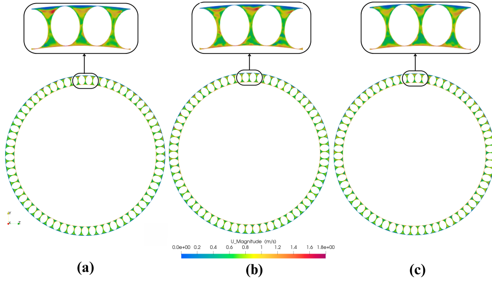
Figure 13. Illustration of velocity fields in MFS row after one rotation of cage (a) 45 % (b) 35 % (c) 21 % grease filling ratio-ratios .
