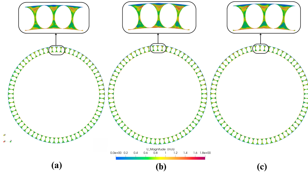
Figure 14. Illustration of velocity fields in HS row after one rotation of cage (a) 45 % (b) 35 % (c) 21 % grease filling ratio-ratios .
