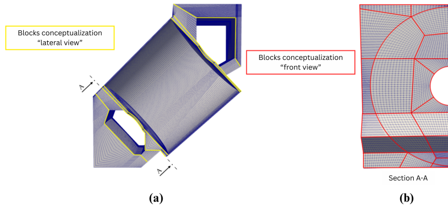
Figure 2. Mesh of the half sector (a) Lateral view (b) Front view.
