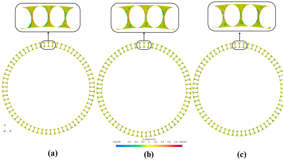
Figure 16. Illustration of axial velocity fields in HS row after one rotation of cage (a) 45 % (b) 35 % (c) 21 % grease filling ratio
