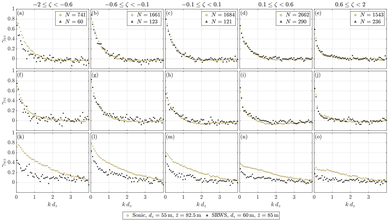
Figure 17. Vertical co-coherence of (a)–(e) along-wind, (f)–(j) cross-wind, and (k)–(o) vertical velocity from sonic anemometers and SRWS at comparable separations and measurement heights under strongly unstable (left) to strongly stable (right) conditions.
