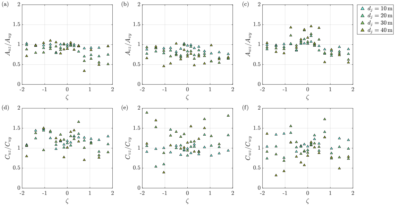
Figure 23. Ratio of vertical to lateral (a)–(c) scaling coefficients and (d)–(f) decay coefficients for separations of d_j = 10\text{m} \dots 40\text{m} d_j = 10\text{m} to 40\text{m} and mean heights of \bar{z} = 120\text{m} \dots 130\text{m} \bar{z} = 120\text{m} to 130\text{m} .
