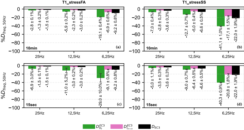
Figure 9. Relative damage loss with respect to 50 Hz at tower section T1 for Fore-Aft (FA) and Side-to-Side (SS), computed by Equation (4)(4). Bars show total, low-frequency, and high-frequency contributions for 25, 12.5, and 6.25 Hz, using 10-minute and 15-second windows. Values are six-month means with standard deviations. Damage computed with EC3 detail category 80 curve.
