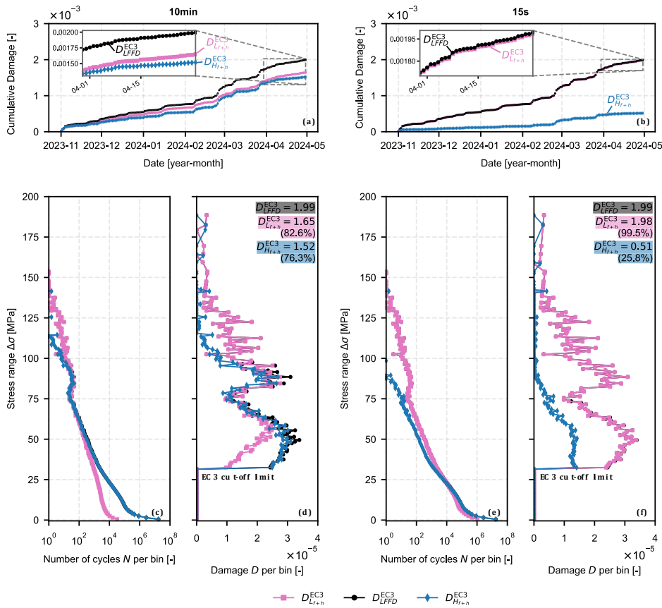
Figure 1244. FA-direction fatigue at tower section T1 (six months, 6.25 Hz): residual-preserving LFFD versus conventional window-based counting. (a-b) Cumulative damage for 10-minute and 15-second windows. (c, e) \Delta\sigma - N spectra and (d, f) \Delta\sigma - D spectra at the end of the six months, for 10-minute and 15-second windows respectively. Curves compare LFFD total damage (baseline), the LFFD low-frequency contribution, and conventional window-based high-cycle counting. Percentages indicate damage relative to the LFFD baseline at tower section T1 (six months, 6.25 Hz). (a-b) Cumulative damage for 10-minute and 15-second windows. (c, e) \Delta\sigma - N spectra and (d, f) \Delta\sigma - D spectra at the end of the six months. Curves compare LFFD total damage (baseline), LFFD low-frequency contribution, Start-Peaks-Valleys-End (SPVE), Max-Min, and conventional window-based high-cycle counting (IEC practice when applied to 10-minute). Percentages indicate total damage relative to the LFFD baseline (Equation (5)(5), EC3). Insets show a zoomed view of the final month of the monitoring period (15-second panel restricted to LFFD total and low-frequency, for clarity). Damage is computed using EC3 detail category 80, employing a bi-linear formulation with slopes m = 3/5 . Damage is computed using EC3 detail category 80, employing a bi-linear formulation with slopes m = 3/5 .
