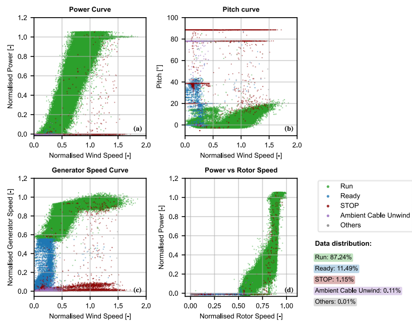
Figure 5. SCADA operational curves for the study period (15-second data). (a-c) Normalised power, pitch, and generator-speed curves versus normalised wind speed. (d) Normalised power versus normalised rotor speed. Colours indicate operational status; the right panel shows the sample distribution by status.
