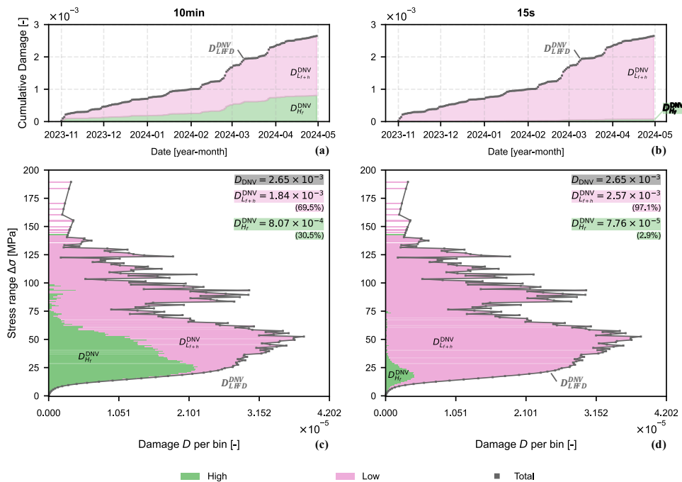
Figure 1140. FA-direction fatigue at tower section T1 (six months, 50 Hz), computed using the DNV welded-steel \sigma - N curve (bi-linear formulation, slopes m = 3/5 ). (a–b) Cumulative damage for 10-minute and 15-second windows. (c–d) Final \Delta\sigma - D spectra. Total damage is decomposed into within-window full-cycle damage (green) and residual-based damage (pink). The percentages of damage are computed by Equation (2)(2). Damage is computed using EC3 detail-category 80 and DNV welded-steel \sigma - N curves, both employing a bi-linear formulation with slopes m = 3/5 .
