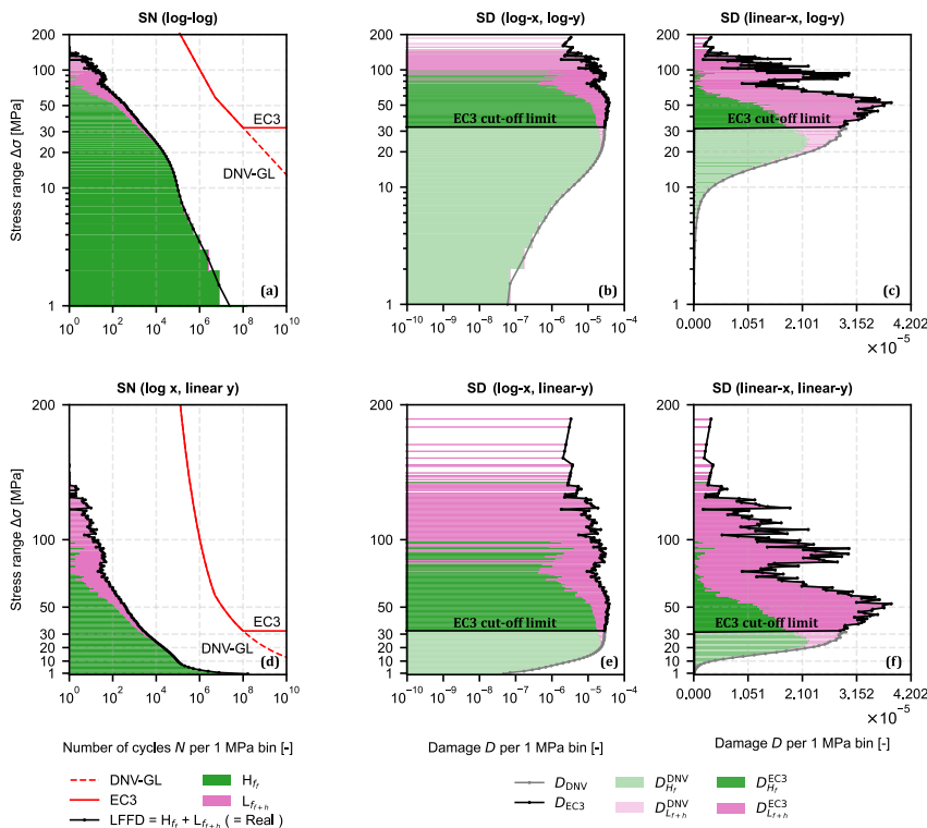
Figure 6. Comparison of \Delta\sigma - N and \Delta\sigma - D fatigue representations for conventional 10-minute windows. Panels (a) and (d) show the \Delta\sigma - N distributions together with the EC3 and DNV \sigma - N curves. The top row (a–c) uses logarithmic scaling on the y-axis, while the bottom row (d–f) uses linear scaling on the y-axis. Panels (b) and (e) present the corresponding \Delta\sigma - D distributions with logarithmic scaling on the x-axis, whereas panels (c) and (f) show the same distributions using linear scaling on the x-axis. Green and pink denote the LFFD high-frequency and low-frequency fatigue contributions, respectively, while the black curve represents the total fatigue distribution.
