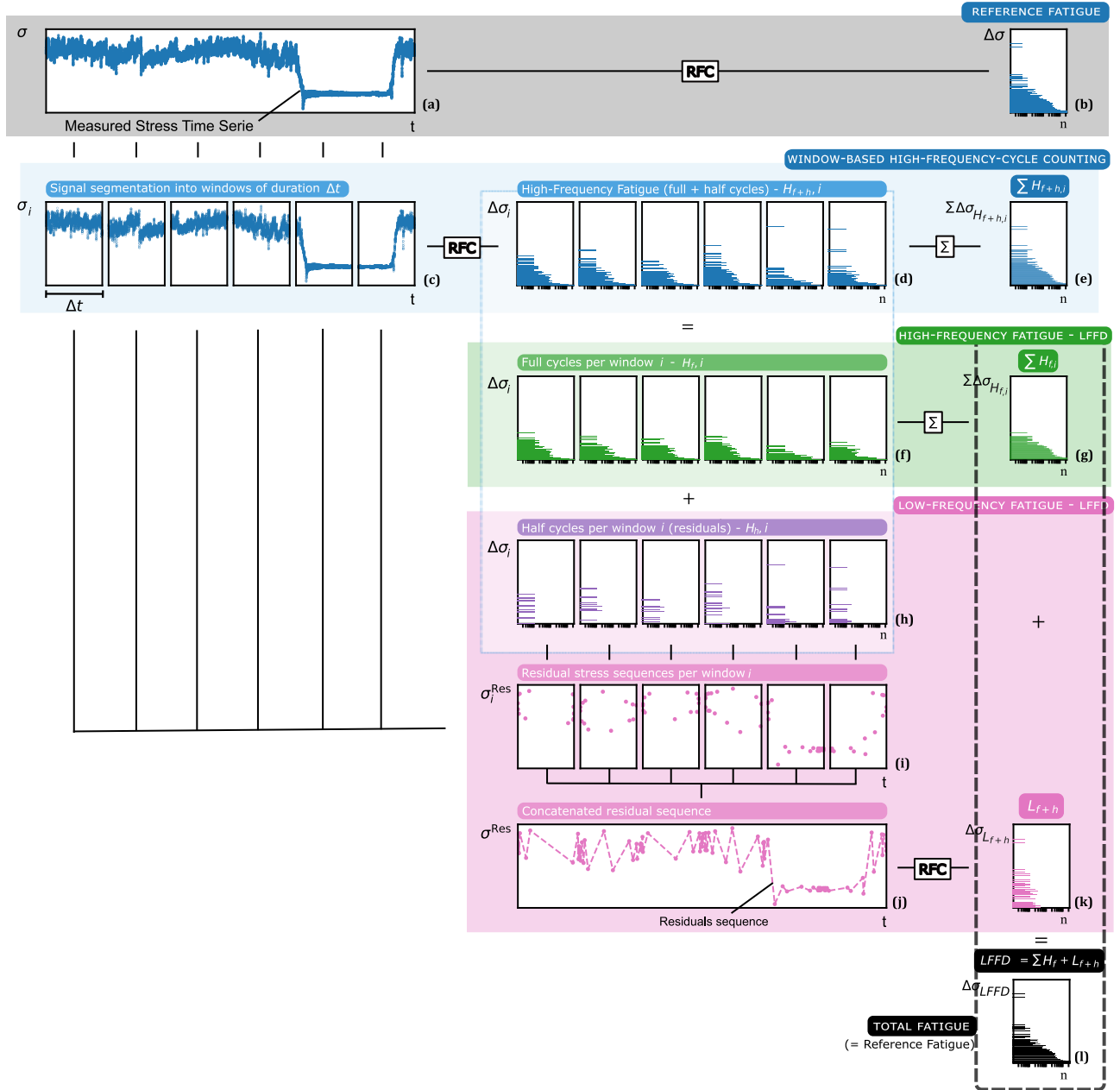
Figure 1. Overview of fatigue monitoring methodologies based on Rainflow Cycle Counting (RFC). (a) Measured stress time series. (b) Baseline fatigue spectrum obtained by applying RFC to the full signal, including full and half cycles. (c) Segmentation of the stress time series into consecutive windows of duration \Delta t . (d) RFC applied independently to each window, yielding window-level fatigue spectra. (e) Aggregated fatigue spectrum obtained by summing full and half cycles across all windows. (f) Full cycles extracted within each window. (g) Aggregated full-cycle spectrum representing the high-frequency, window-contained fatigue contribution. (h) Half cycles remaining in each window. (i) Residual stress sequences associated with unclosed half cycles. (j) Concatenation of residual stress sequences across windows. (k) RFC applied to the concatenated residual sequence, capturing low-frequency fatigue cycles spanning multiple windows. (l) Total fatigue spectrum obtained by combining the high-frequency (full-cycle) and low-frequency (residual-based) contributions, preserving equivalence with continuous RFC.
