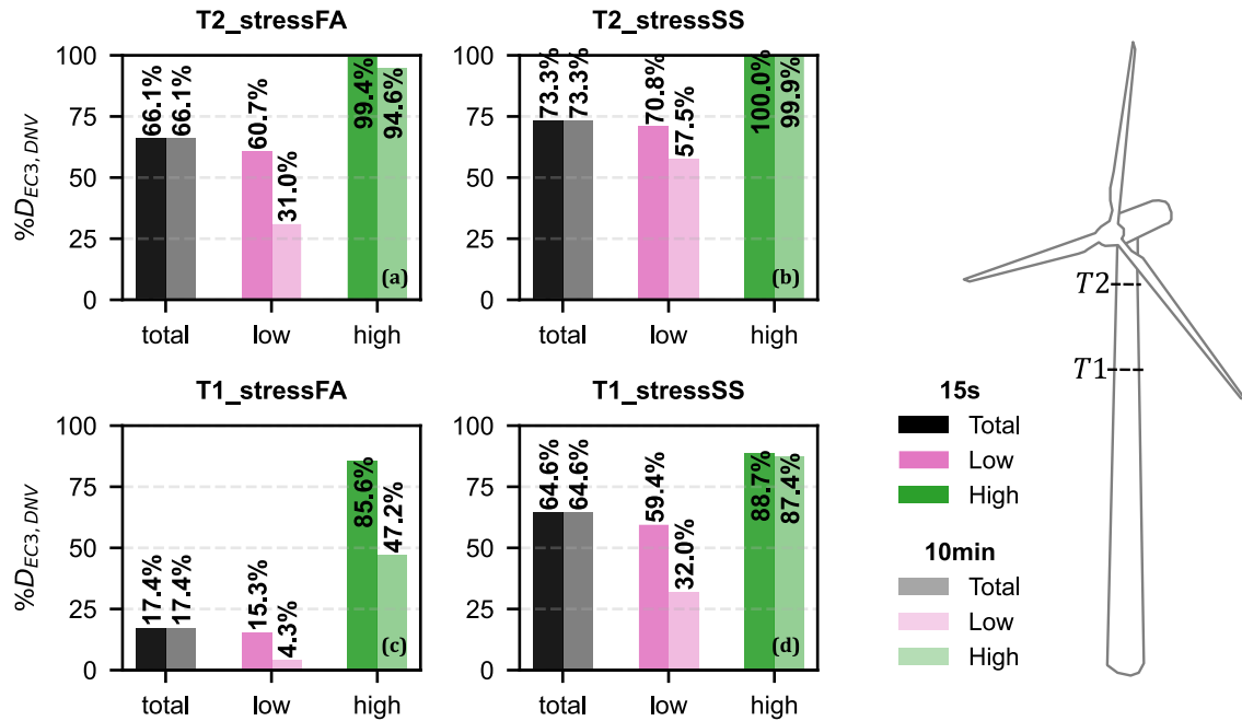
Figure 7. Relative differences between fatigue damage estimates obtained using Eurocode 3 (EC3) and DNVGL-RP-C203 (DNV) for 10-minute and 15-second windows. Damage is computed using EC3 detail category 80 and DNVGL-RP-C203 welded-steel \sigma - N curves, both employing a bi-linear formulation with slopes m = 3/5 . Results are shown for tower section T1 (near-base) and T2 (upper tower) in the fore-aft (FA) and side-to-side (SS) directions: (a) T2-FA, (b) T2-SS, (c) T1-FA, (d) T1-SS. Bars indicate percentage differences in accumulated damage between EC3 and DNV for the total fatigue damage and for the low- and high-frequency contributions, computed using Equation (3).
