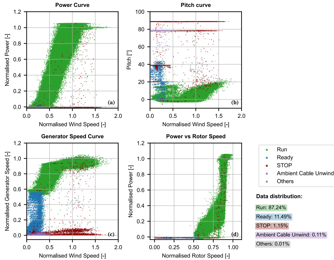
315 Figure 5. SCADA operational curves for the study period (15-second data). (a-c) Normalised power, pitch, and generator-speed curves versus normalised wind speed. (d) Normalised power versus normalised rotor speed. Colours indicate operational status; the right panel shows the sample distribution by status.
