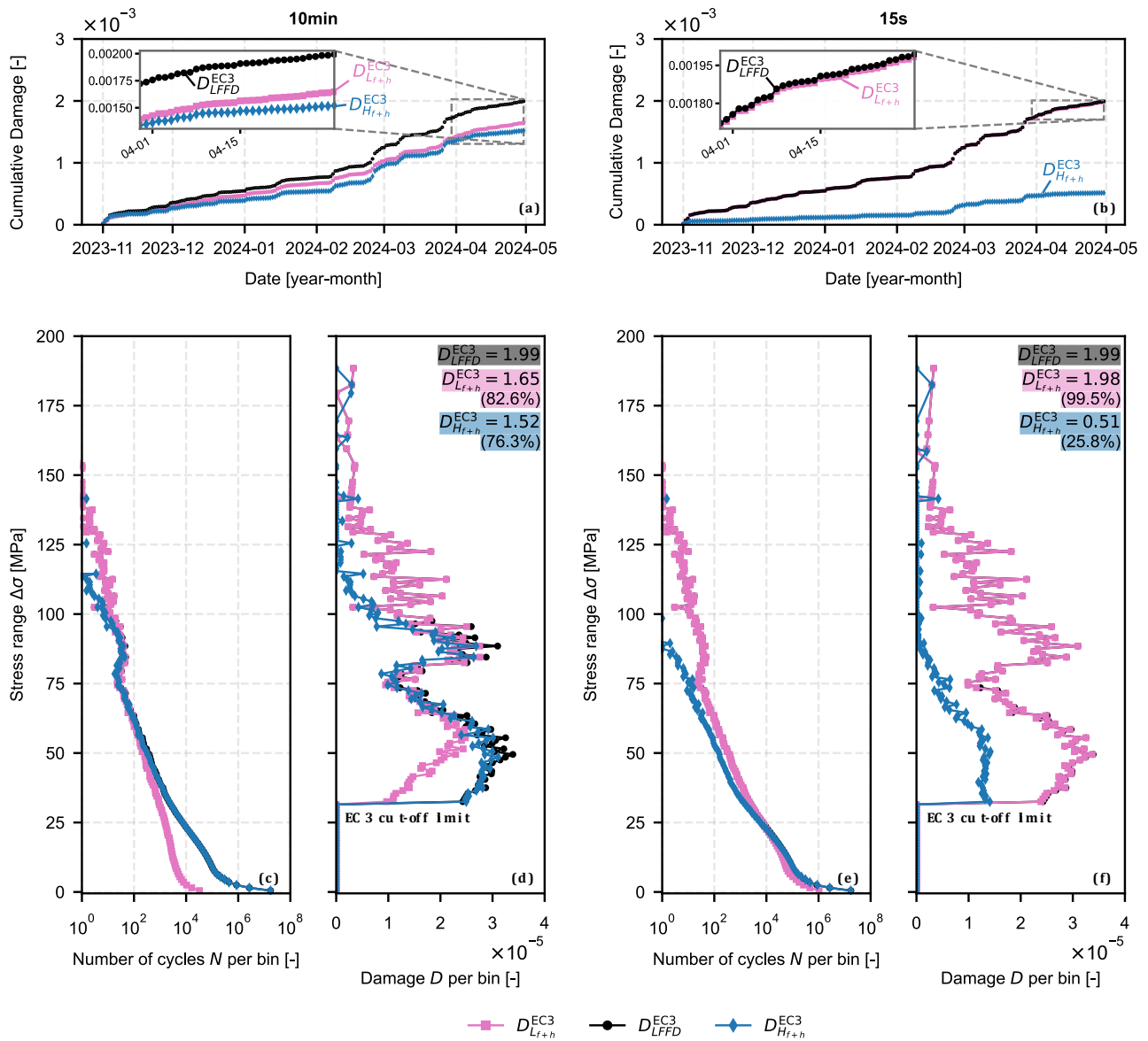
Figure 12. FA-direction fatigue at tower section T1 (six months, 6.25 Hz): residual-preserving LFFD versus conventional window-based counting. (a–b) Cumulative damage for 10-minute and 15-second windows. (c, e) \Delta\sigma - N spectra and (d, f) \Delta\sigma - D spectra at the end of the six months, for 10-minute and 15-second windows respectively. Curves compare LFFD total damage (baseline), the LFFD low-frequency contribution, and conventional window-based high-cycle counting. Percentages indicate damage relative to the LFFD baseline (Equation (5), EC3). Insets show a zoomed view of the final month of the monitoring period (15-second panel restricted to LFFD total and low-frequency, for clarity). Damage is computed using EC3 detail category 80, employing a bi-linear formulation with slopes m = 3/5 .
