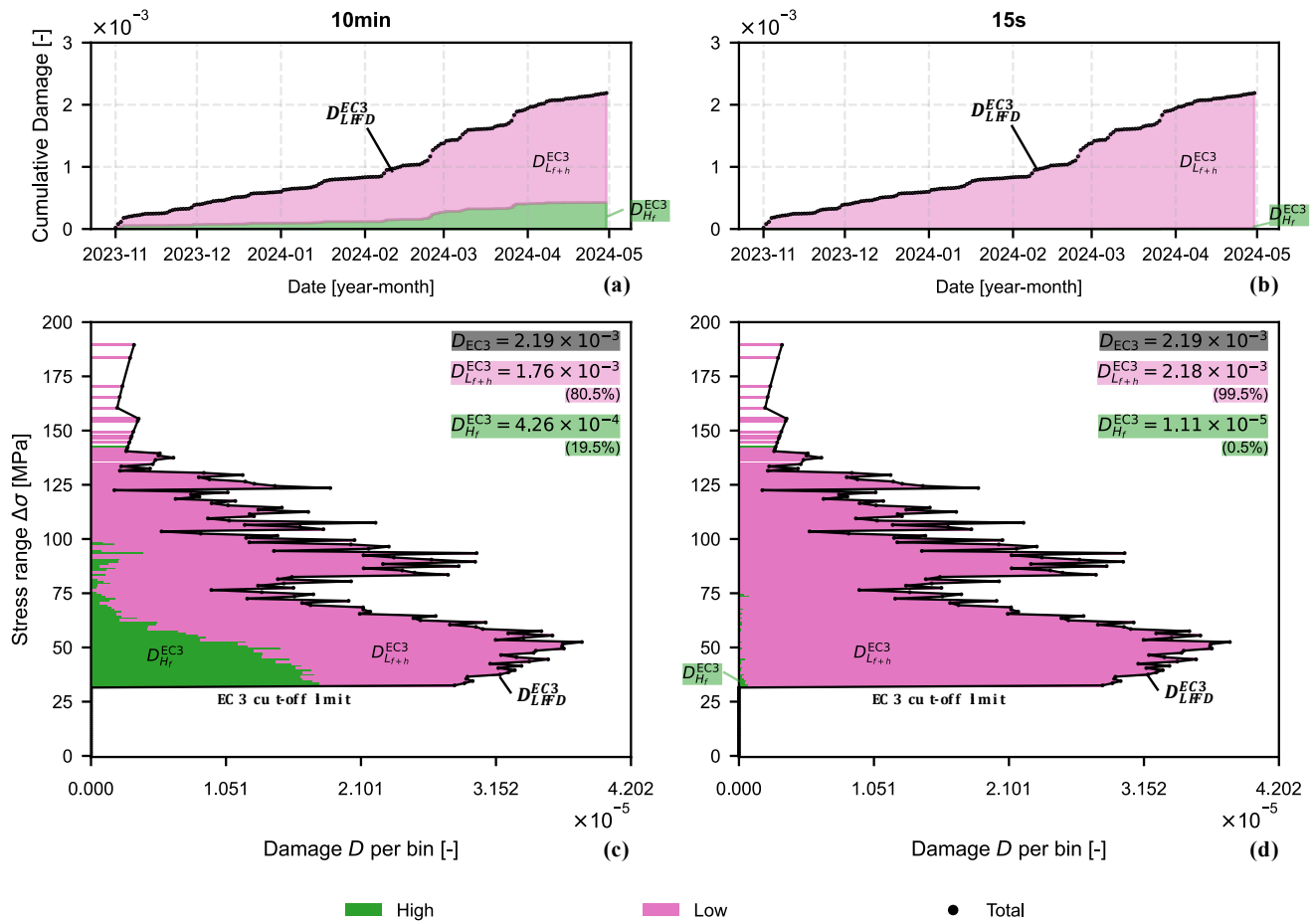
Figure 10. FA-direction fatigue at tower section T1 (six months, 50 Hz), computed using the EC3 detail category 80 \sigma - N curve (bi-linear formulation, slopes m = 3/5 ). (a–b) Cumulative damage for 10-minute and 15-second windows. (c–d) Final \Delta\sigma - D spectra. Total damage is decomposed into within-window full-cycle damage (green) and residual-based damage (pink). The percentages of damage are computed by Equation (2).
