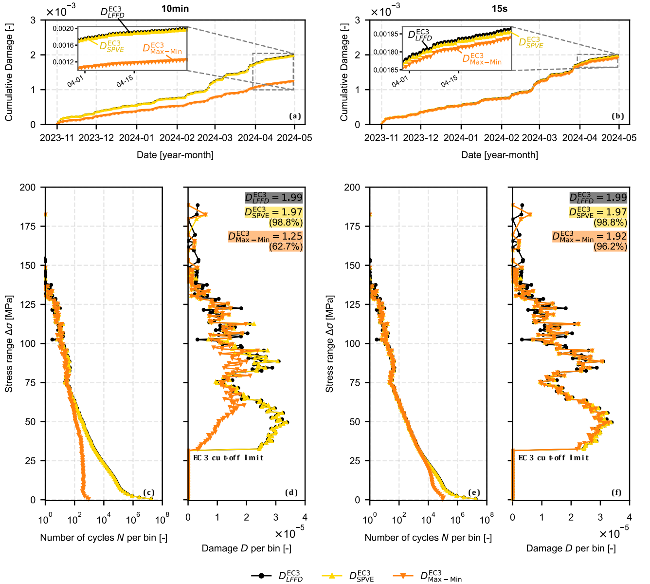
Figure 13. FA-direction fatigue at tower section T1 (six months, 6.25 Hz): LFFD baseline versus reduced-information extrema representations. (a–b) Cumulative damage for 10-minute and 15-second windows. (c, e) \Delta\sigma - N spectra and (d, f) \Delta\sigma - D spectra at the end of the six months, for 10-minute and 15-second windows respectively. Curves compare LFFD total damage (baseline), Start–Peaks–Valleys–End (SPVE), and Maximum–Minimum (Max–Min). Percentages indicate damage relative to the LFFD baseline (Equation (5), EC3). Insets show a zoomed view of the final month of the monitoring period. Damage is computed using EC3 detail category 80, employing a bi-linear formulation with slopes m = 3/5 .
