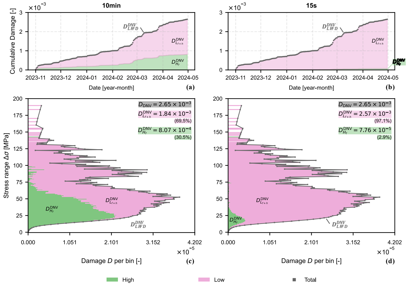
Figure 11. FA-direction fatigue at tower section T1 (six months, 50 Hz), computed using the DNV welded-steel \sigma - N curve (bi-linear formulation, slopes m = 3/5 ). (a–b) Cumulative damage for 10-minute and 15-second windows. (c–d) Final \Delta\sigma - D spectra. Total damage is decomposed into within-window full-cycle damage (green) and residual-based damage (pink). The percentages of damage are computed by Equation (2).
