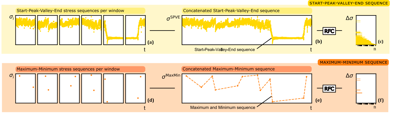
Figure 3. Extrema sequence methods for reduced-information fatigue assessment. (a) Windowed extraction of start, peaks, valleys, and end (SPVE) points within each window. (b) Concatenation of the windowed SPVE values to form a continuous start–peaks–valleys–end sequence; Rainflow Cycle Counting (RFC) is applied to identify fatigue cycles, including those spanning multiple windows. (c) Resulting fatigue spectrum obtained from the SPVE sequence. (d) Windowed extraction of maximum and minimum stress values per window. (e) Concatenation of windowed maxima and minima to form a maximum–minimum (Max–Min) sequence; Rainflow Cycle Counting (RFC) is applied to identify fatigue cycles. (f) Resulting fatigue spectrum obtained from the Max–Min sequence. The SPVE approach preserves local turning-point structure, while the Max–Min approach provides a highly compressed representation emphasising large-amplitude, long-period stress variations.
