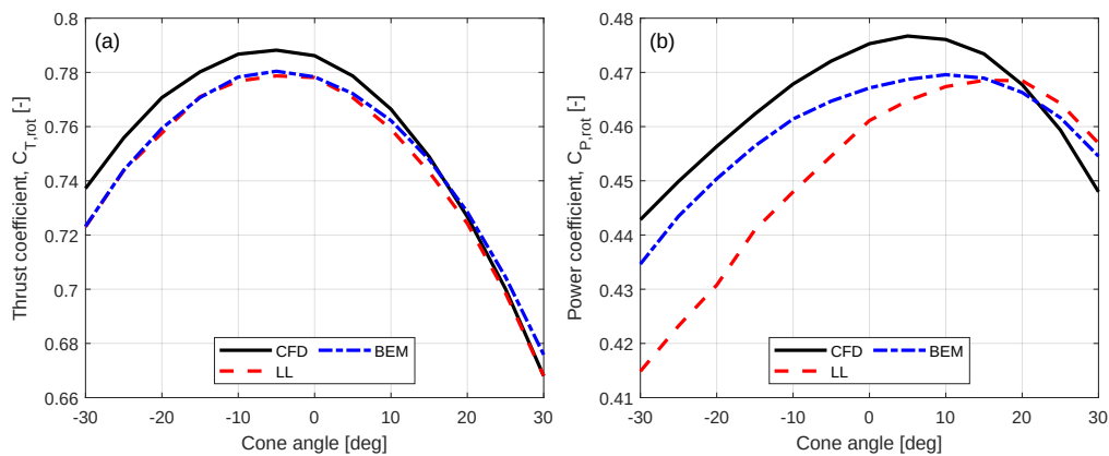
Figure 3. Rotor-integrated (a) thrust coefficient C_{T,\text{rot}} and (b) power coefficient C_{P,\text{rot}} as functions of cone angle for EllipSys3D CFD, MIRAS LL, and the HAWC2 BEM formulation. The LL and BEM calculations use fully turbulent airfoil polars.
