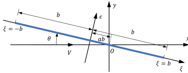
Figure 1. Definitions of the flow and airfoil coordinate systems and positive directions used in the derivation of unsteady 2-D thin-airfoil theory. Adapted from Li et al. (2022) with permission.
