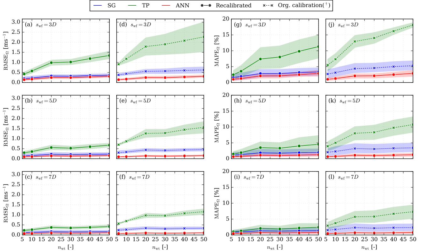
Figure 6. Flow study result metrics for an increasing number of wind turbines, without a blockage model. (a-c) RMSE_{\Omega} with calibrated recalibrated wake models, (d-f) RMSE_{\Omega} with uncalibrated for the wake models with original parameters , (g-i) MAPE_{\Omega} with calibrated recalibrated wake models, and (j-l) MAPE_{\Omega} with uncalibrated wake models using the original parameters .
