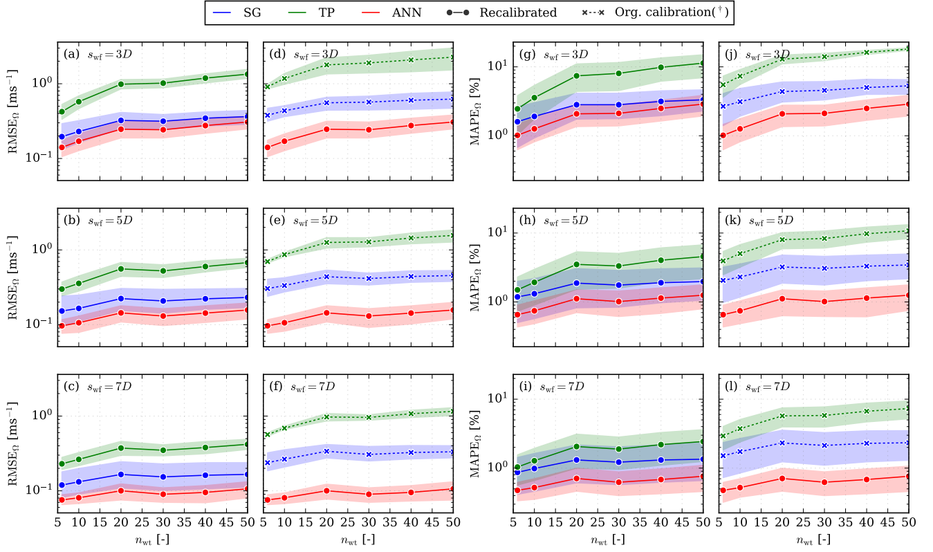
Figure C1. Flow study result metrics for an increasing number of wind turbines, without a blockage model displayed on a semi-logarithmic axis. Containing the same data as Fig. 6.
