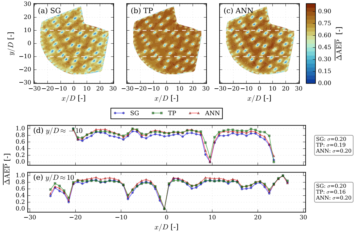
Figure D1. Objective function maps illustrating the normalized AEP improvement \overline{\Delta AEP} for the calibrated low-fidelity models without blockage: (a) SG model, (b) TP model, (c) ANN model with a cross-plane profile for all models (d) at y/D \approx -10 , and (e) at y/D \approx 10
