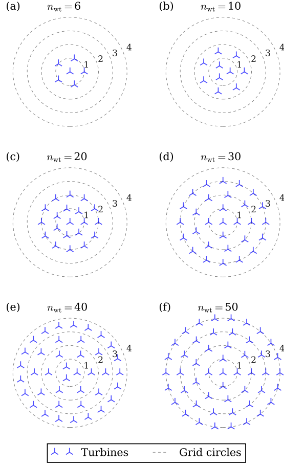
Figure 3. Circular turbine layouts evaluated in the wind farm flow study. The grid circles represent normalized radial positions, which are scaled by a separation factor s_{\text{wf}} \in \{3D, 5D, 7D\} to generate configurations with varying inter-turbine spacing.
