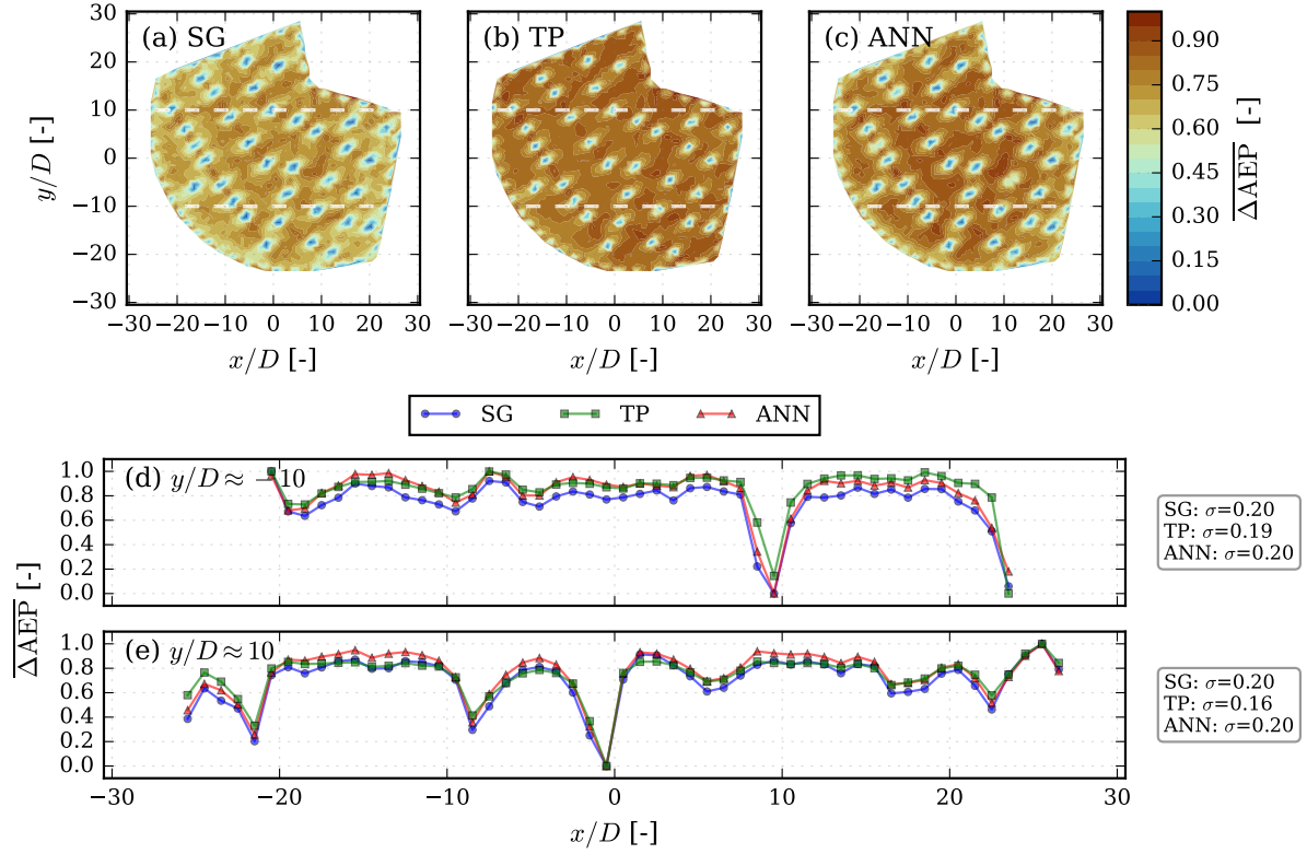
Figure D1. Objective function maps illustrating the normalized AEP improvement \overline{\Delta AEP} for the calibrated low-fidelity models without blockage: (a) SG model, (b) TP model, (c) ANN model with a cross-plane profile for all models (d) at y/D \approx -10 , and (e) at y/D \approx 10
