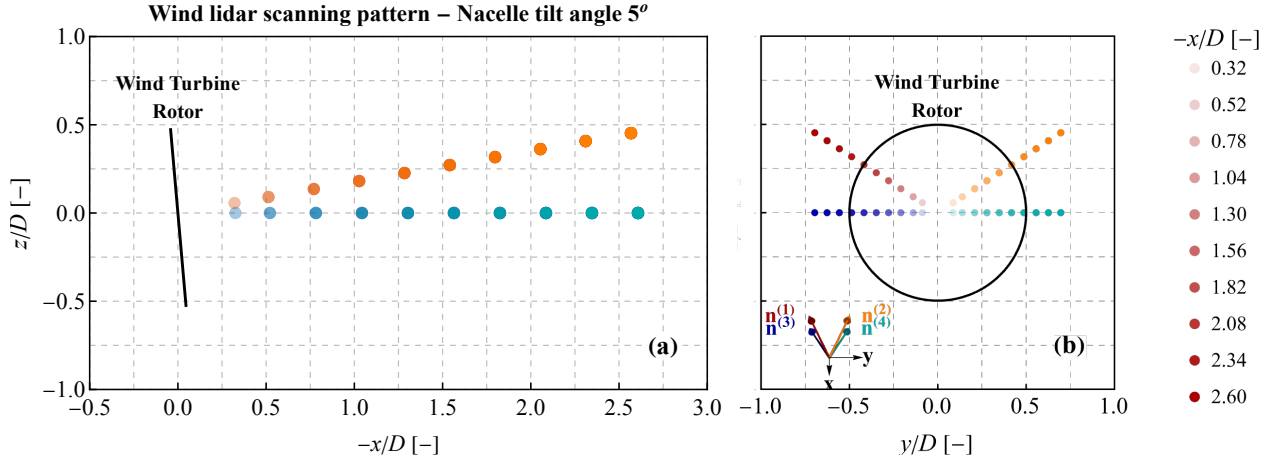
Figure 2. Scanning pattern of the nacelle-mounted wind lidar when the tilt of the floating offshore wind turbine was is equal to 5^\circ , corresponding to the wind speed ranges 8.5 - 9.5 \text{ ms}^{-1} and 12.5 - 13.5 \text{ ms}^{-1} . The two lower beams (denoted as n^{(3)} and n^{(4)} ) are almost horizontal when the pitch angle is approximately equal to 5^\circ . The x -axis is parallel to the yaw direction and pointing downwind.
