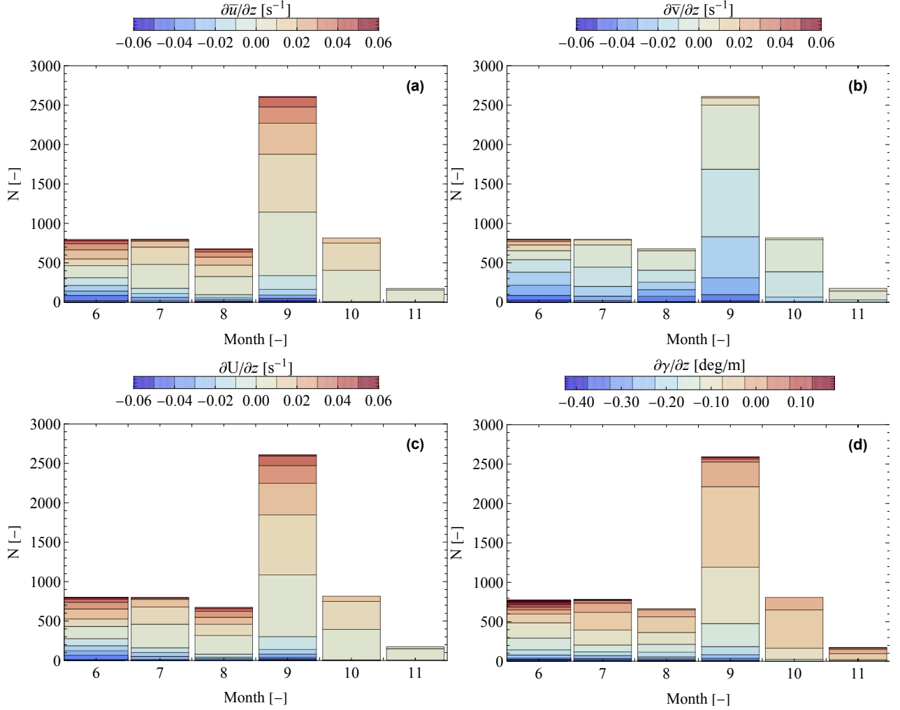
Figure 4. Bar chart of the distribution of the estimated wind-shear-gradients (a) \frac{\partial \bar{u}}{\partial z} and (b) veer \frac{\partial \bar{v}}{\partial z} along with the corresponding shear (c) and veer (d) of the wind profile along the top part of the wind turbine rotor for different 10-minute periods over different months.
