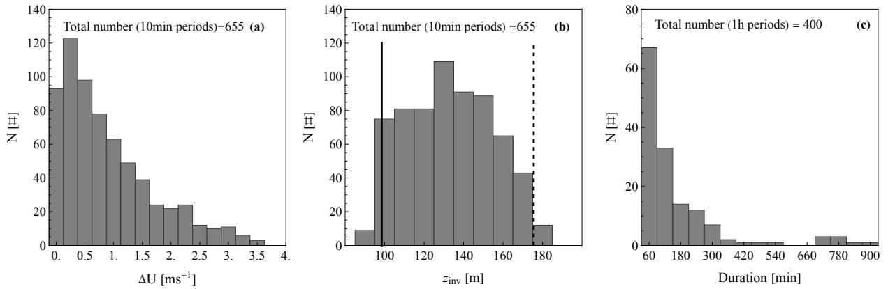
Figure 6. Duration, the height Histograms of the wind speed inversion ( z_{\text{inv}} ) and the wind speed difference ( \Delta U ) between the maximum and the minimum wind speed along the wind vertical profile, (b) the height of the wind speed inversion ( z_{\text{inv}} ) and (c) the duration of periods in which either wind speed inversion or negative shear were identified. The solid and dashed vertical lines in (b) denote the hub height and top height of the rotor.
