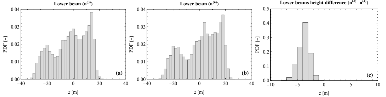
Figure B1. Probability density function of the height z of the range gate measurement of 2.6 D of the left (a) and right (b) lower beams of the nacelle-mounted Doppler lidar in relation to the hub-height and (c) of the difference between the two.
